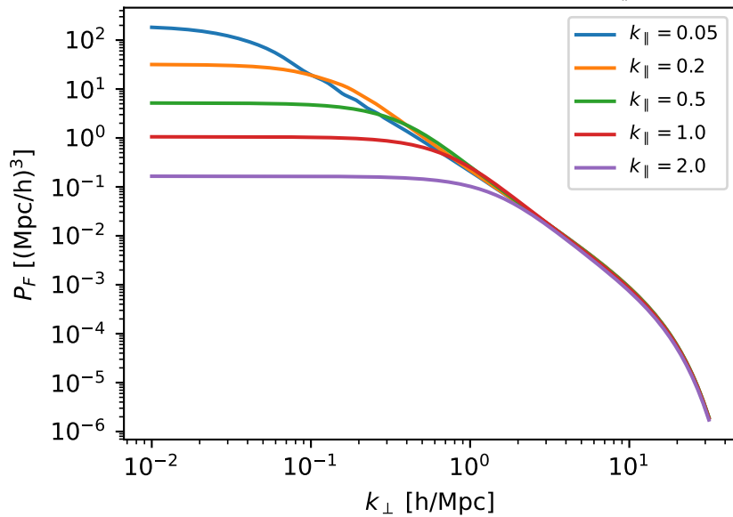
transverse shape at fixed k_{\parallel}
