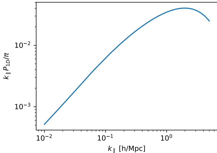
fiducial P1D ( z=2.4 )
