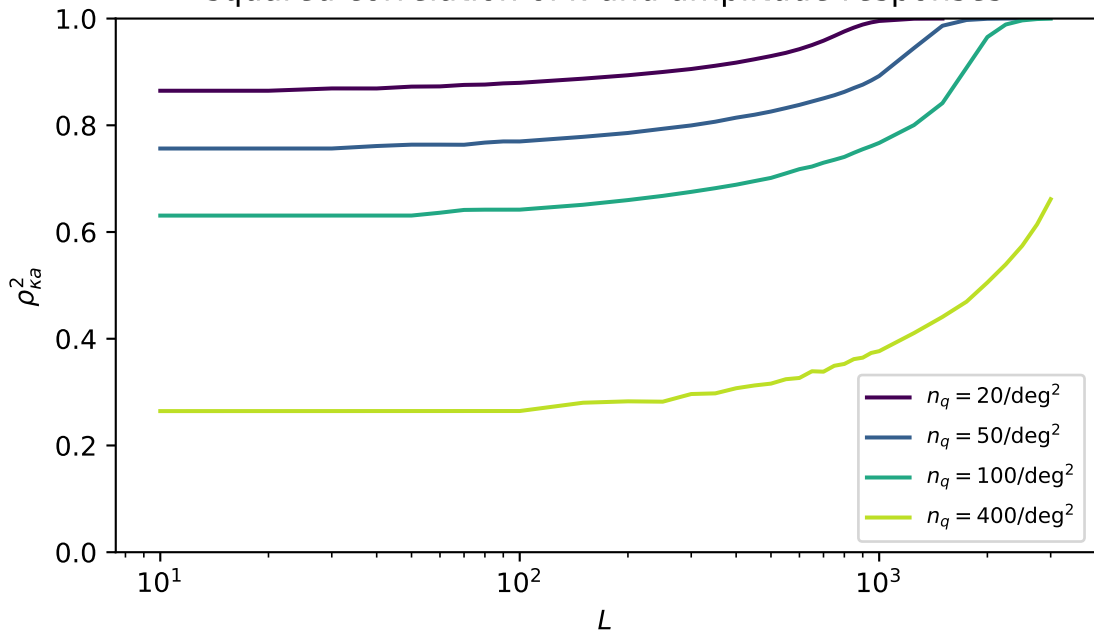
squared correlation of \kappa and amplitude responses
