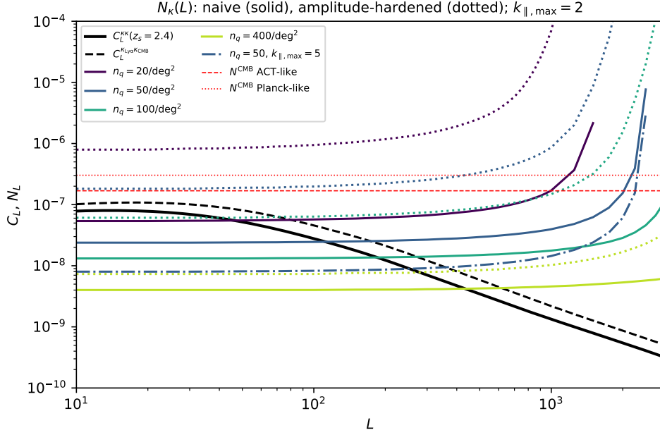
Figure 2: Sample-variance-limited reconstruction noise N_\kappa(L) (solid, Eq. 15) for sightline densities n_q and k_{\parallel, \max} = 2 h \text{ Mpc}^{-1} , its per-screen amplitude-hardened version (dotted, Eq. 16), and the case k_{\parallel, \max} = 5 for n_q = 50 (dash-dotted). Black curves are the forest convergence auto-spectrum and its cross-spectrum with \kappa_{\text{CMB}} ; red lines are the white-noise equivalents of the ACT DR6 and Planck PR4 reconstruction noise.
