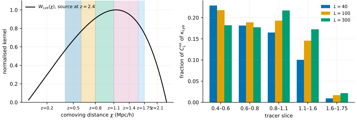
Figure 1: Left: the lensing kernel of a source at z = 2.4 (the effective forest redshift) with the tracer slices of the first version ( 0.4 < z < 1.75 ) shaded; the 0.1–0.4 slice of this version sits below them. Right: the fraction of the power of \kappa_{\text{Ly}\alpha} contributed by each slice at L = 40, 100 and 300 (Limber, non-linear matter power); the slices together hold 69–77 per cent.
