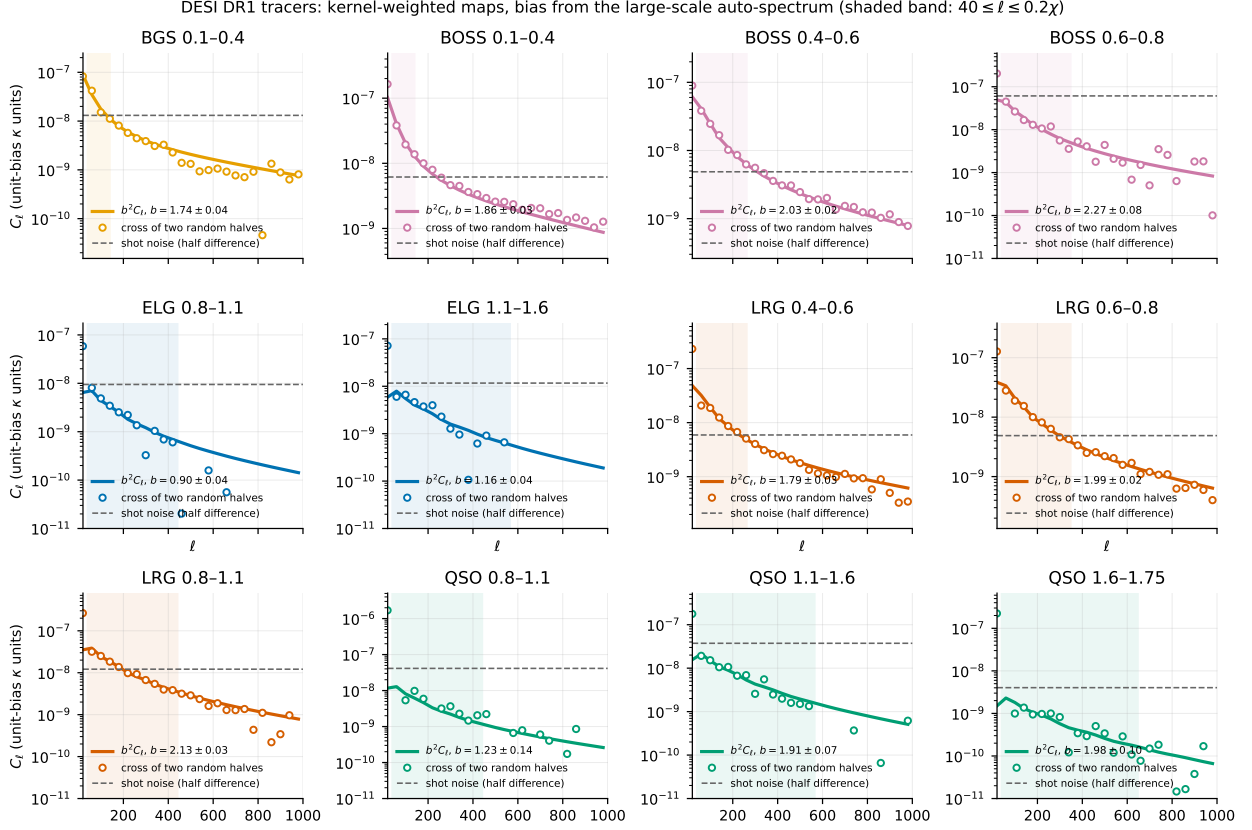
Figure 5: Angular power spectra of the twelve tracer maps in convergence units for unit bias: the NaMaster cross-spectrum of two random halves (points, no shot noise), the fitted b^2 C_\ell through the bandpower windows (line) and the shot noise measured from the half difference (dashed). The shaded band is the fit range 40 \leq \ell \leq 0.2\chi(z_{\text{mid}}) .
