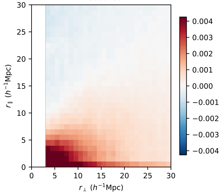
measured
