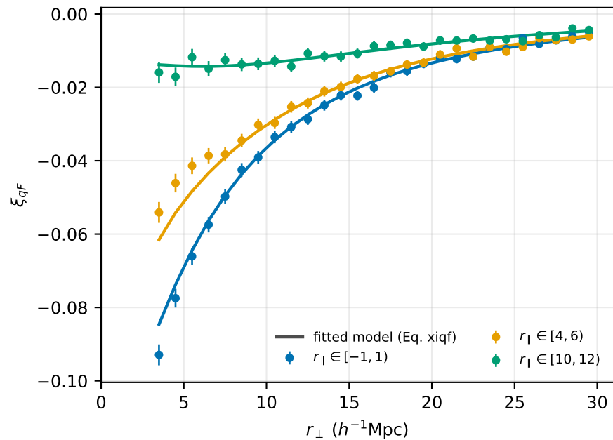
quasar \times forest ( \chi^2 = 5729 for 11340 cells)
