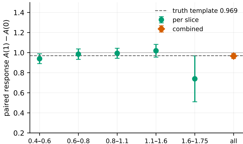
Mock validation (400 realisations, 400 deg 2 , lognormal tracers of the same realisation)
