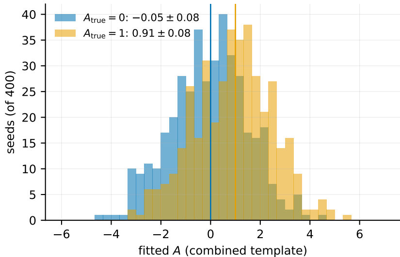
Mock validation (400 realisations, 400 deg 2 , lognormal tracers of the same realisation)
