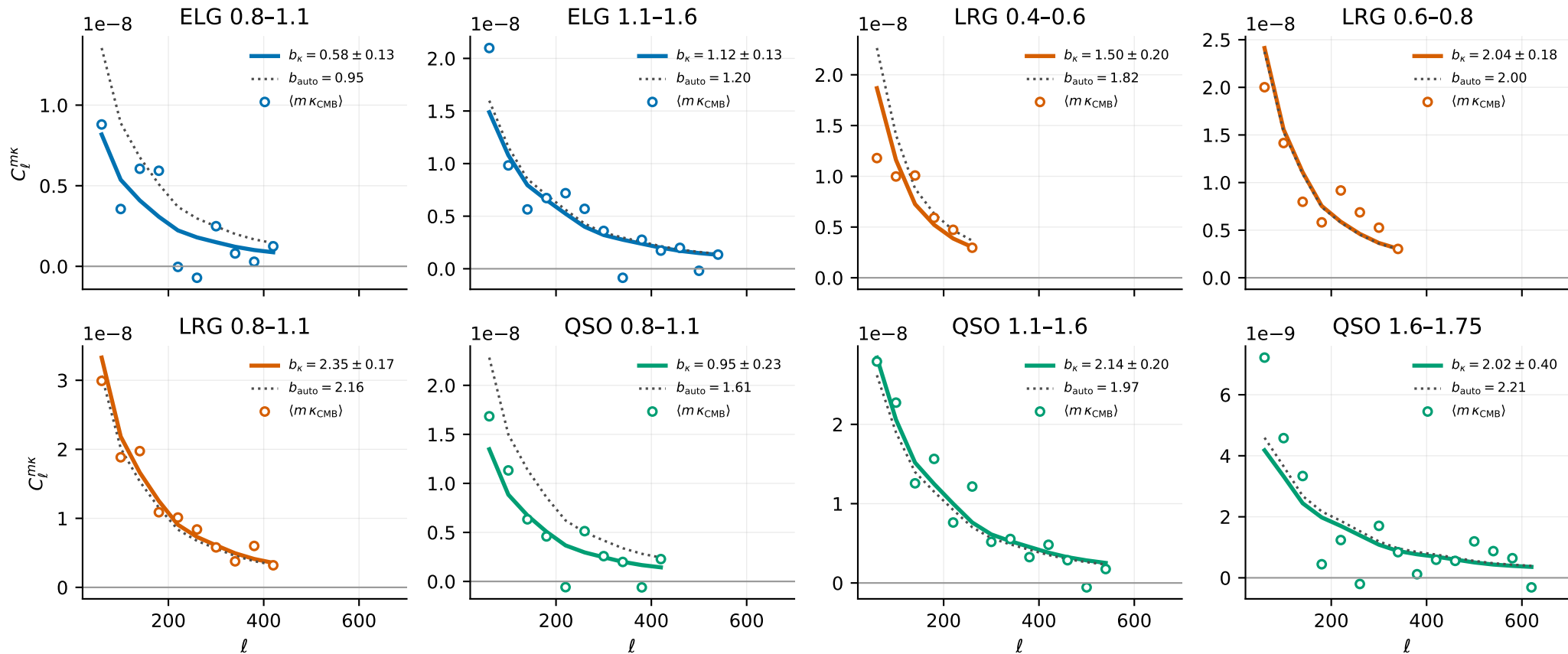
Cross-spectra of the tracer maps with the ACT DR6 lensing map (joint sky fraction 0.05–0.08)
