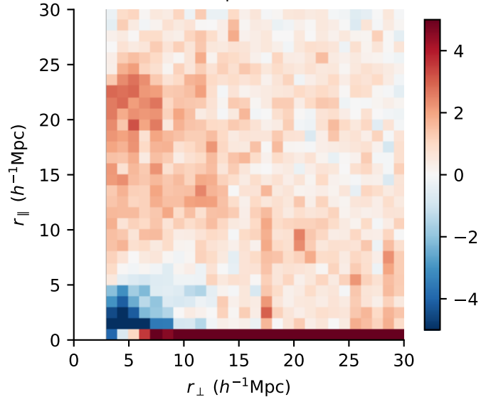
residual / \sigma , two-parameter Kaiser fit
