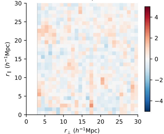
residual / \sigma , with the spline correction
