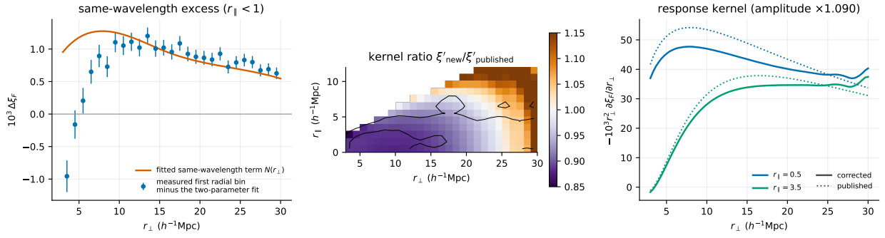
Figure 3: What the correction does. Left: the excess of the first radial bin over the two-parameter fit (points) and the fitted same-wavelength term N(r_{\perp}) (line); it is flat at \simeq 10^{-3} beyond 6 h^{-1} \text{Mpc} and enters the mean field but not the kernel. Middle: the ratio of the new response kernel to the one used in the first measurement, over the part of the pair domain where the kernel is large, with contours of the Fisher-information density of the amplitude. Right: the kernel itself, -r_{\perp}^2 \partial \xi_F / \partial r_{\perp} , at two radial separations, published (dotted) against corrected (solid). Fisher-weighted, the kernel change raises the lensing amplitude by 10 per cent.
