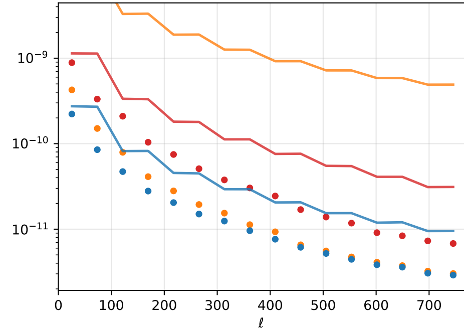
\sigma(\hat{C}_\ell^{\delta M4E}) band (1000, 1500)
