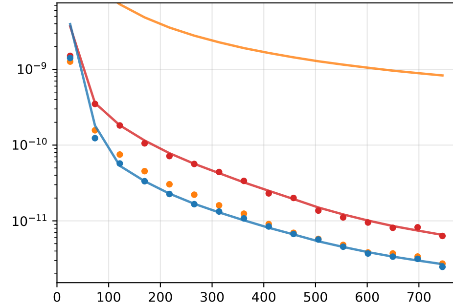
\sigma(\hat{C}_\ell^{\delta M4E}) band (1000, 1500)
