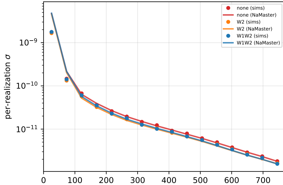
\sigma(\hat{C}_\ell^{\delta M4E}) band (50, 500)
