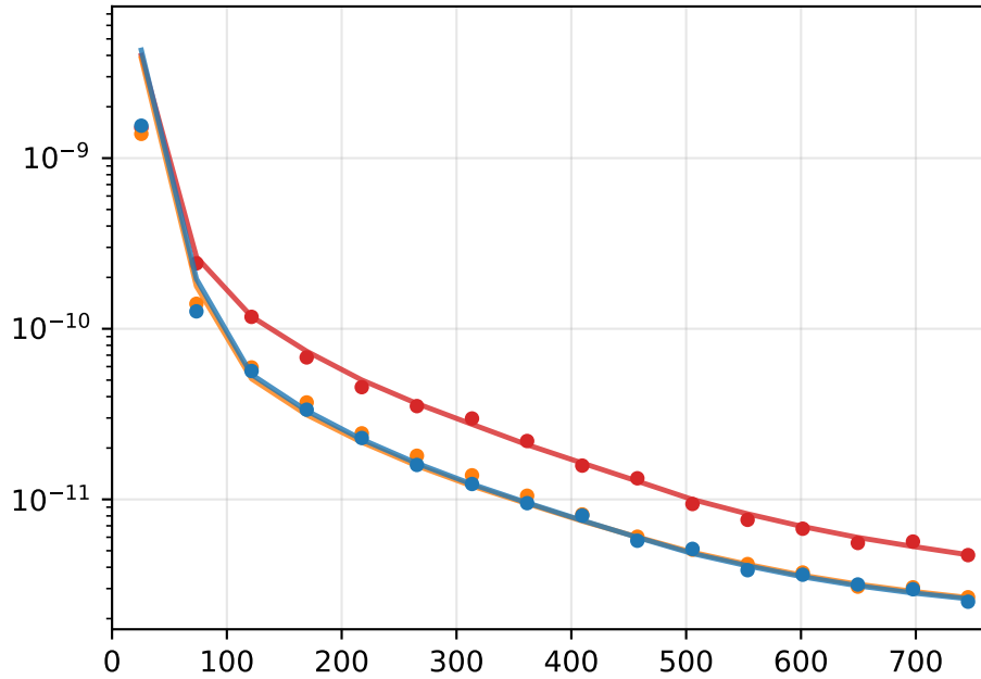
\sigma(\hat{C}_\ell^{\delta M4E}) band (500, 1000)
