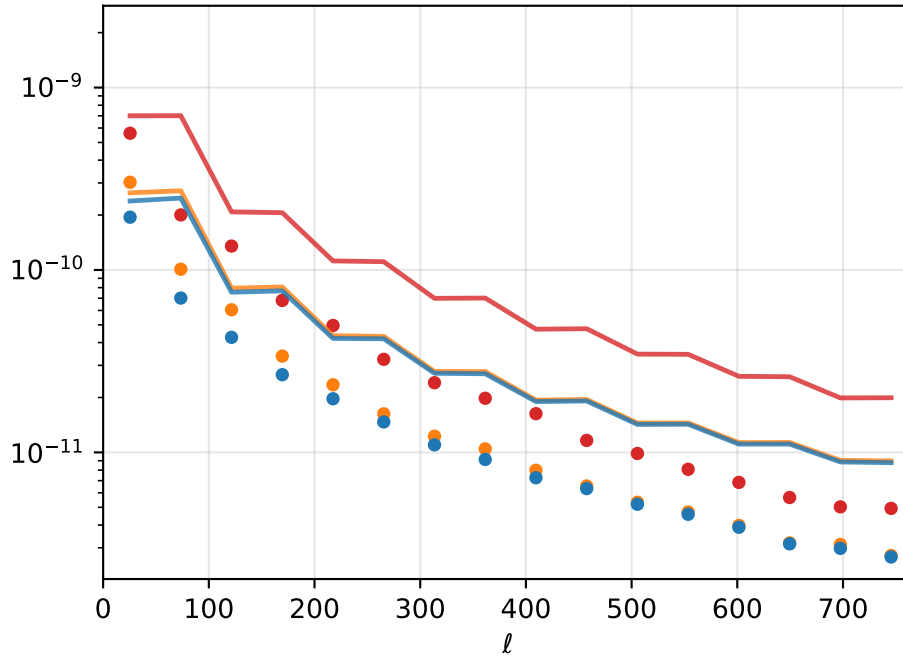
\sigma(\hat{C}_\ell^{\delta M4E}) band (500, 1000)
