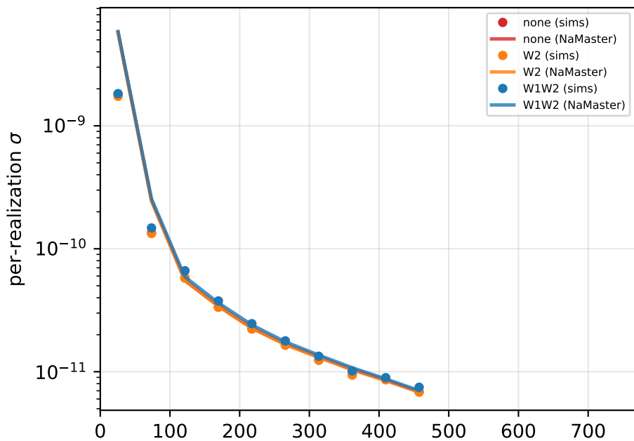
\sigma(\hat{C}_\ell^{\delta M4E}) band (50, 500)
