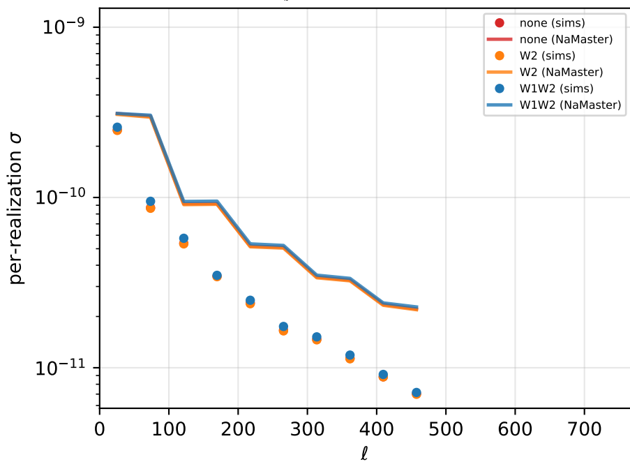
\sigma(\hat{C}_\ell^{\delta M4E}) band (50, 500)
