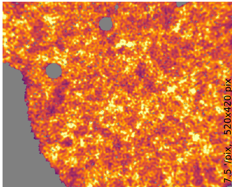
numerical \langle M_0 \rangle_{\text{noise}}
