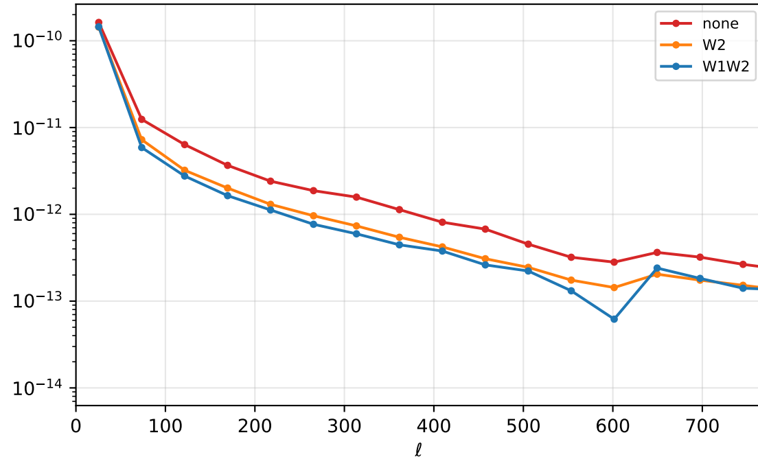
M_0 error on the mean, band (500, 1000)
