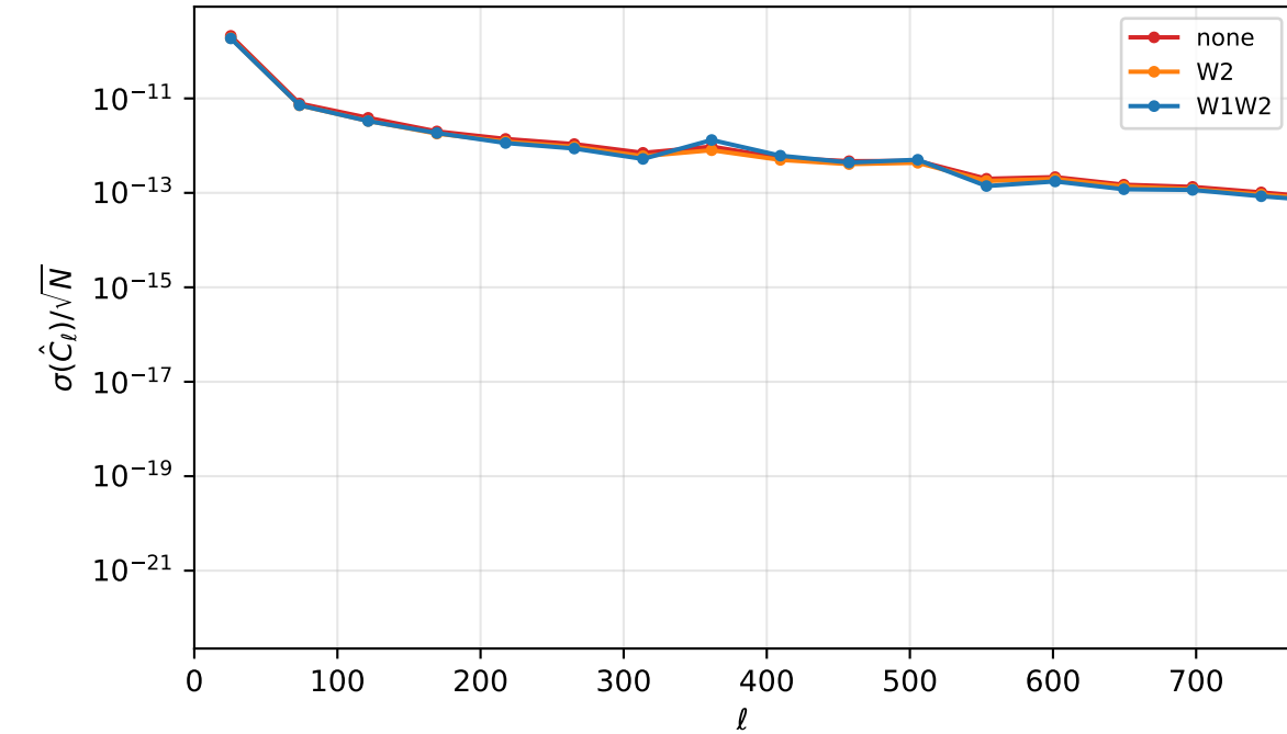
M_0 error on the mean, band (50, 500)
