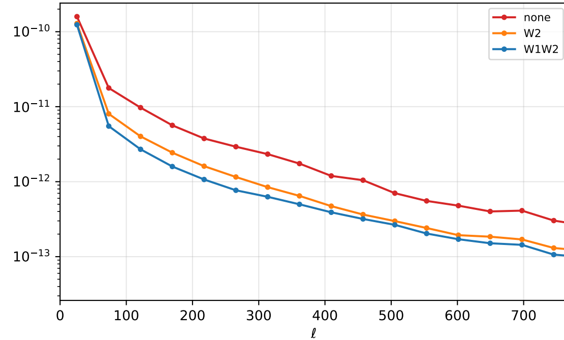
M_0 error on the mean, band (1000, 1500)
