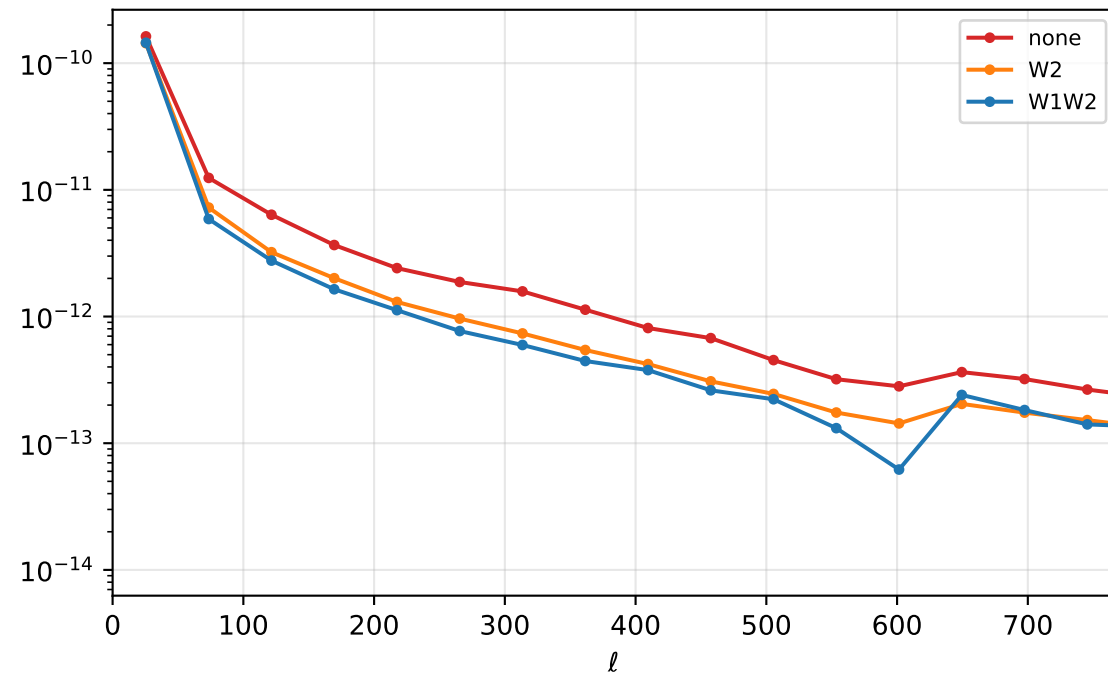
M_0 error on the mean, band (500, 1000)
