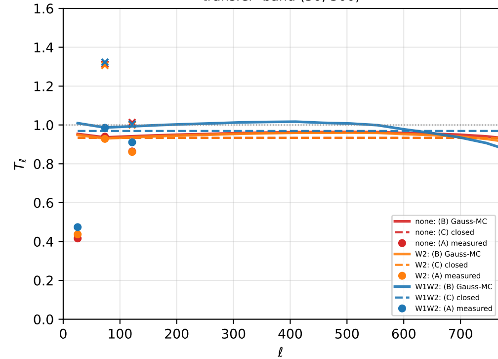
transfer band (50, 500)
