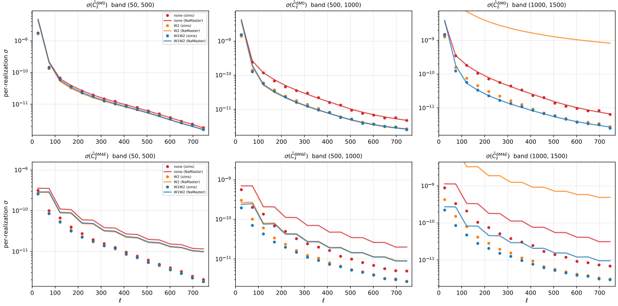
Figure 12: Per-realization error \sigma = \sqrt{\text{diag } \hat{C}} from the 400-realization sample scatter (points) versus the NaMaster Gaussian covariance (lines), for the three schemes and three bands, for M_0 (top) and M_{4E} (bottom). For the spin-0 M_0 cross the two agree to a few percent (cf. Table 4; the lone outlier is the orange line in [1000, 1500], the peaked unwhitened-W2 weight). For the spin-4 M_{4E} cross the Gaussian estimate runs parallel to the sample \sigma (the \ell -shape and scheme ordering match) but high by a near-constant factor \approx 3 : the f_{\text{sky}} = \langle w^2 \rangle deconvolution of the input auto-spectra is cruder for spin-weighted fields, whose mask coupling loses more power than the scalar \langle w^2 \rangle captures. In both channels the error drops from none (red) through W2 (orange) to W1W2 (blue) in the noise-dominated bands — the SNR gain of Table 3. The sample covariance (which is what the analysis uses) is robust for both.
