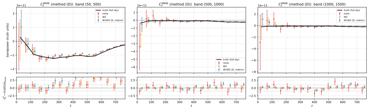
Figure 11: As Fig. 10 for the spin-4 cross \hat{C}_\ell^{\delta M_{4E}} , with the W1W2 channel matrix-decoupled per method (D).
