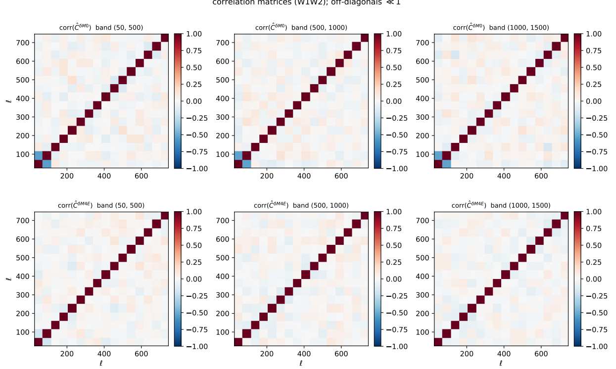
Figure 13: Correlation matrices C_{\ell\ell'}/\sqrt{C_{\ell\ell}C_{\ell'\ell'}} of the 400-realization covariance for the W1W2 scheme, for M_0 (top) and M_{4E} (bottom) in the three bands. The matrices are nearly diagonal; the only visible off-diagonal feature is a mild anti-correlation of the two largest-scale bandpowers.
