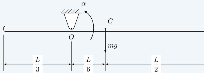
Uniform bar and the forces at release.
