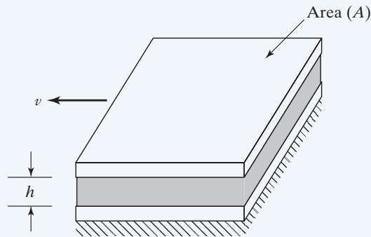
Flat-plate approximation of a lubricant film.
