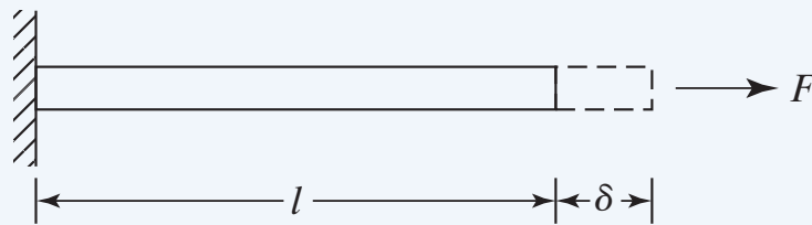
Axial force and end deformation of a uniform rod.
