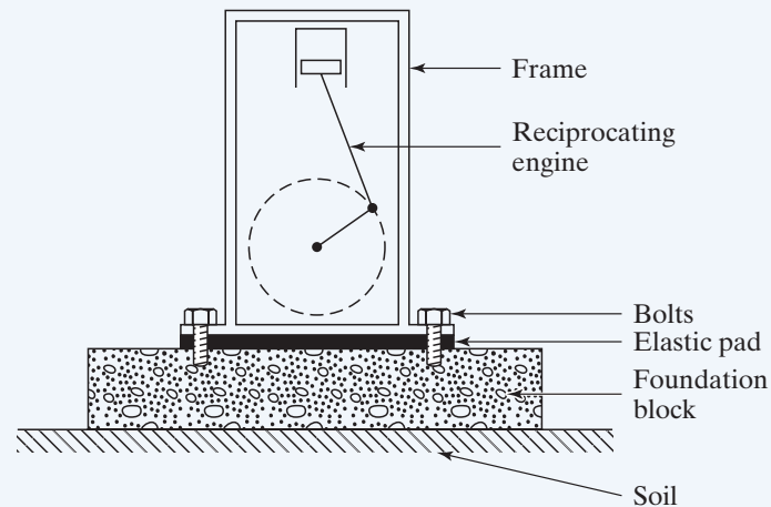
Figure 1.63. A reciprocating engine on a foundation.
