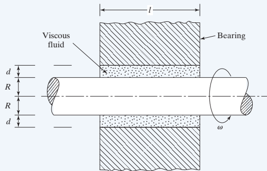
Rotating shaft and surrounding lubricant film.
