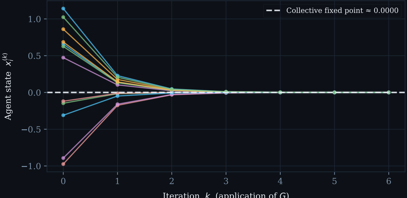
Fig 1 — Multi-Agent Convergence under G^6 ( N = 12 agents, \alpha = 0.3 , \varepsilon = 0.15 )
