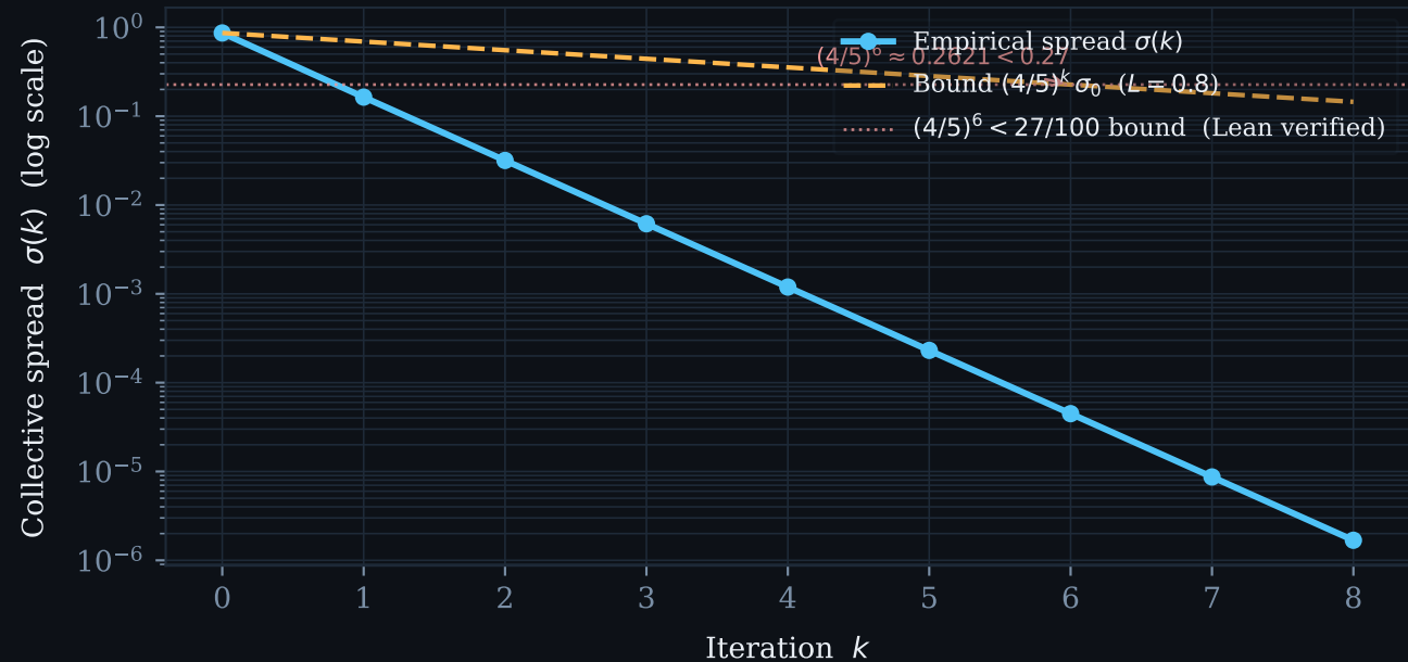
Fig 3 — Contraction of Collective State under G^k ( N = 30 agents, \alpha = 0.3 < 1/2 )
