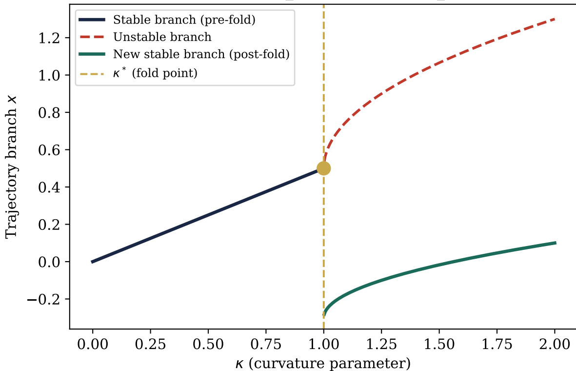
Bifurcation Diagram near \kappa^* Lean: FoldOp.has_fold, FoldOp.finite_branch
