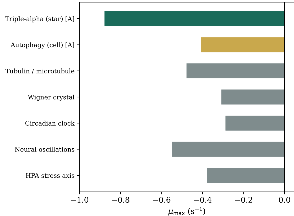
Transverse Lyapunov Exponent Lean: \mu_{\text{dm3\_neg}} (all < 0)
