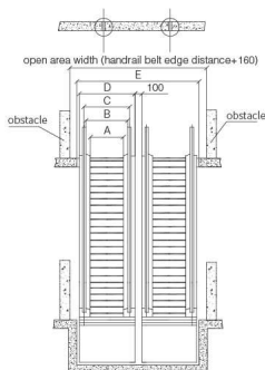
Safety Protection of Escalator Entrances and Exits
