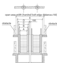
Safety Protection of Escalator Entrances and Exits
