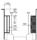
Safety Protection of Escalator Entrances and Exits
