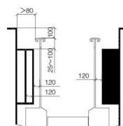
Safety Protection of Escalator Entrances and Exits
