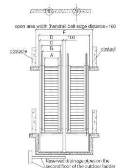
Safety Protection of Escalator Entrances and Exits
