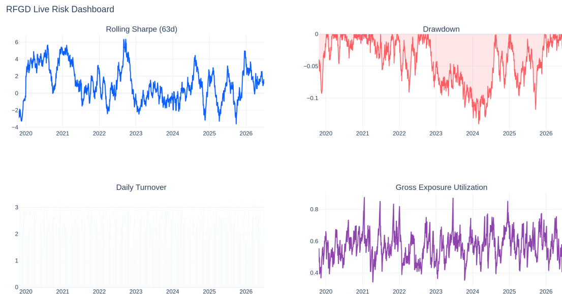
Figure 8.4: Four-panel live risk dashboard: rolling 63-day Sharpe ratio, drawdown, daily turnover, and gross exposure utilization under the 10% annualized volatility target. This is the exact chart format generated nightly by the production monitoring pipeline.
