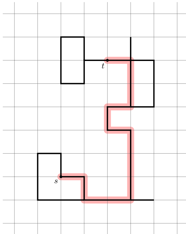
FIGURE 1 – Un labyrinthe
