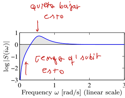
(a) Bode integral formula
