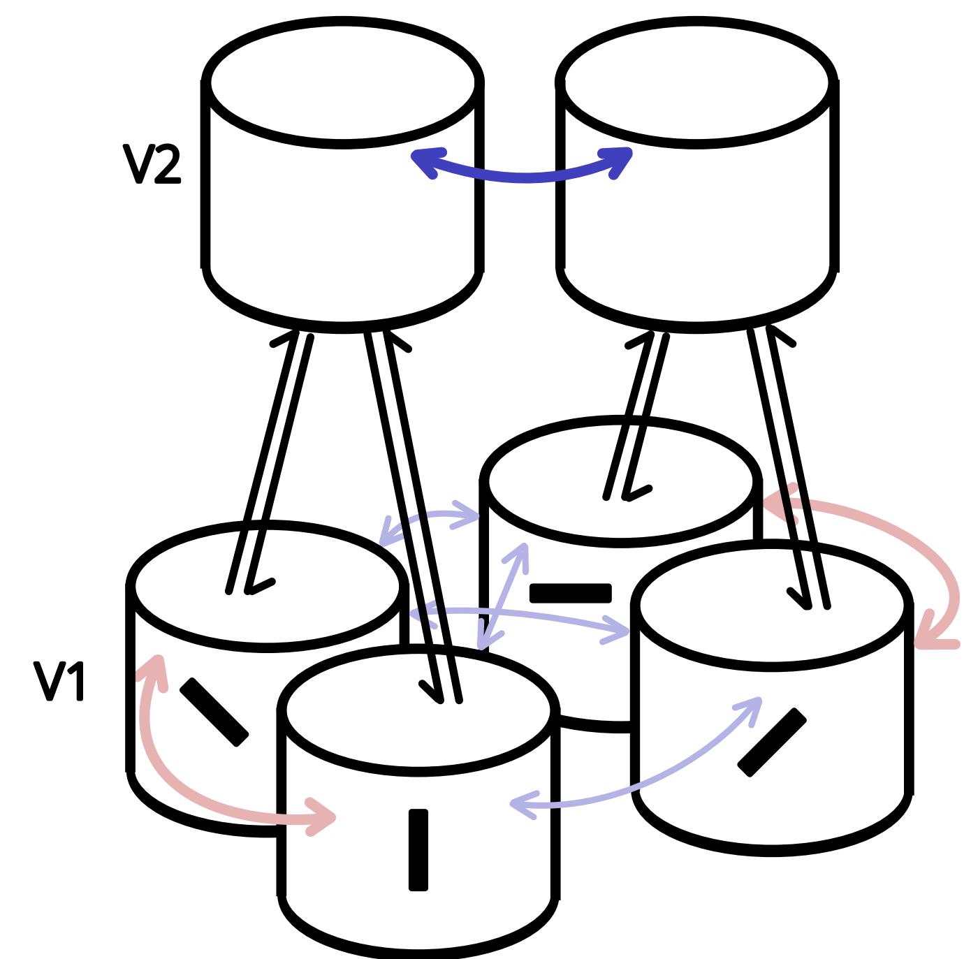
With feedforward and feedback from V1 to V2, and lateral inhibition in V1 and V2
