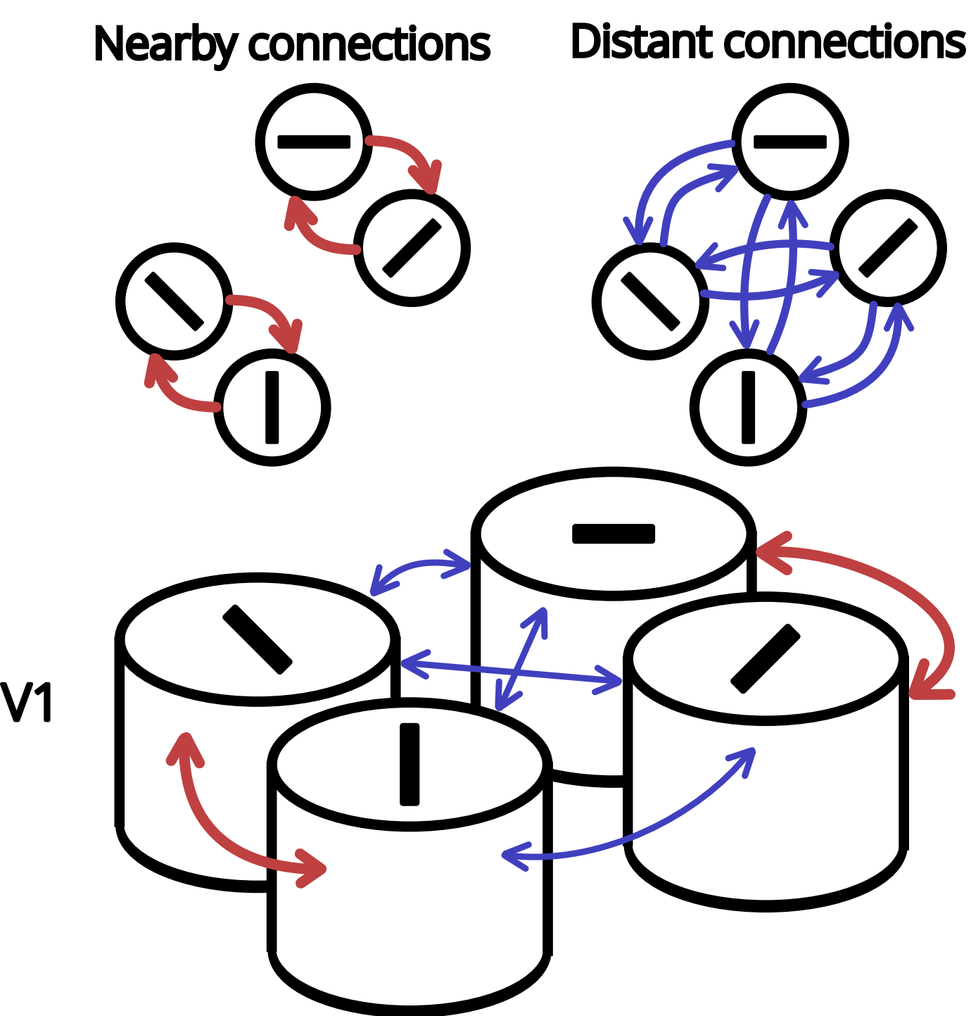
With lateral inhibition in V1 only
