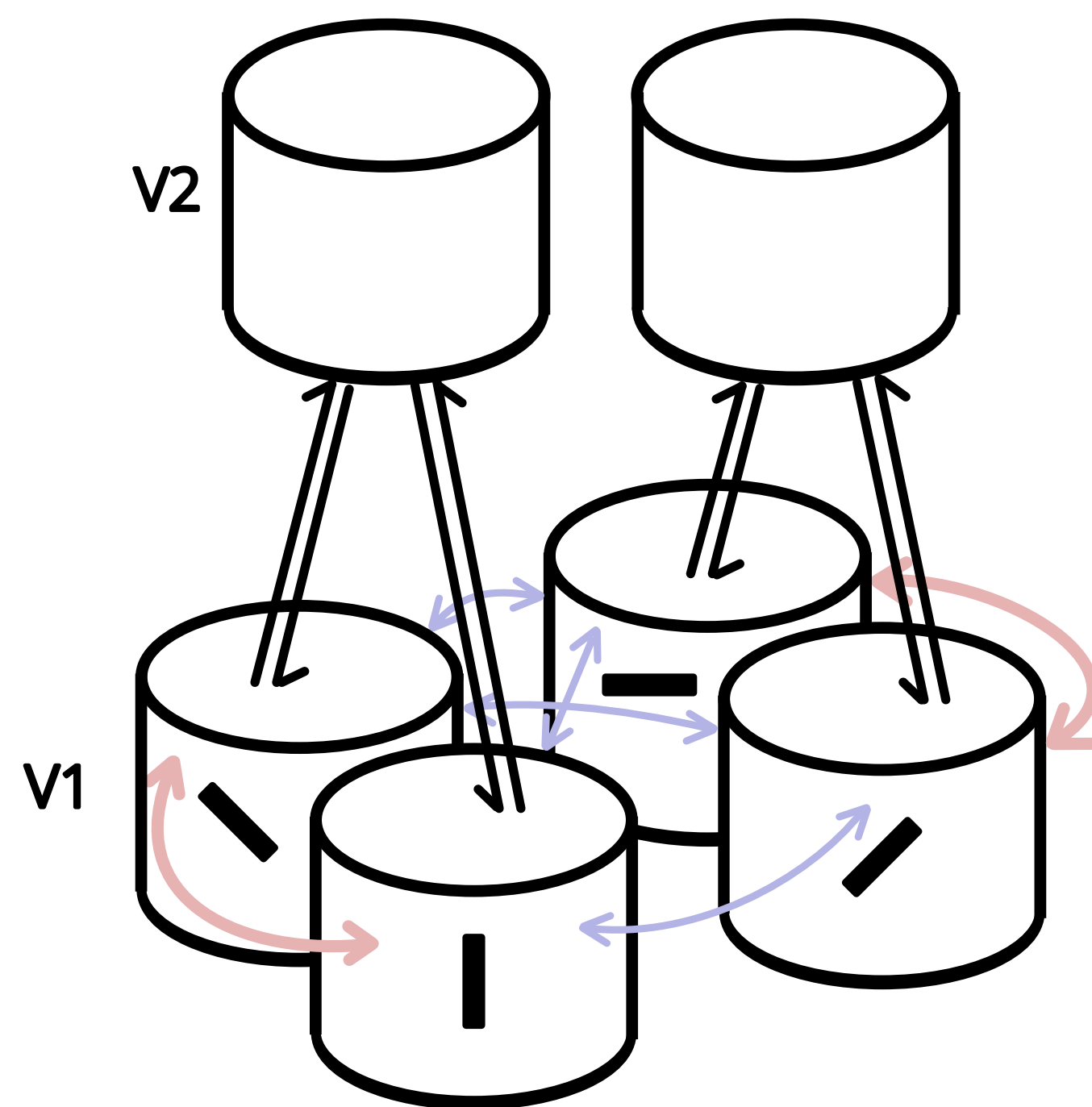
With feedforward and feedback from V1 to V2, and lateral inhibition in V1
