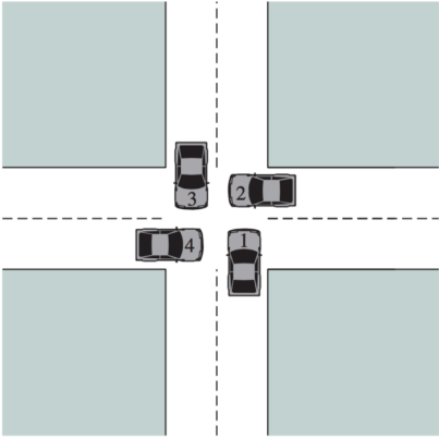
(b) Deadlock
