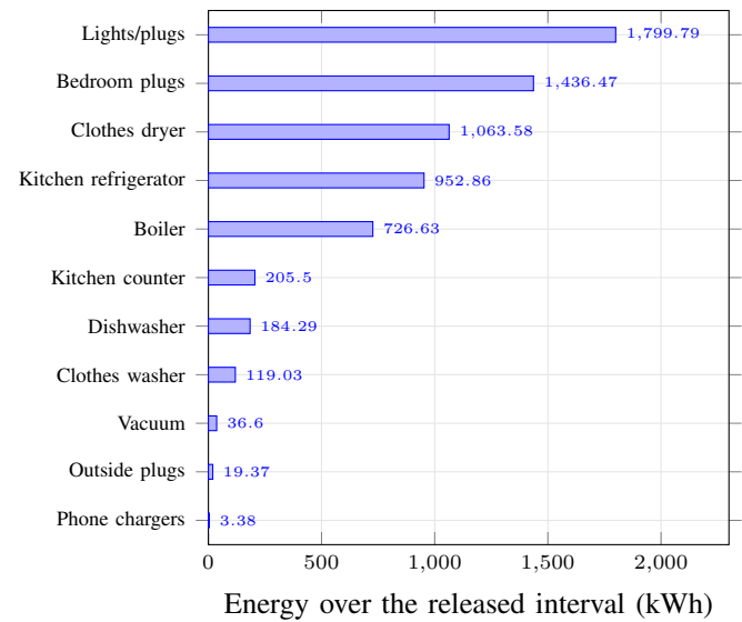
FIG. 2. Non-overlapping component energy from the 18 non-main logical channels, grouped by description. Values are kWh. The utility and main aggregates are deliberately excluded to avoid double counting downstream circuits.
