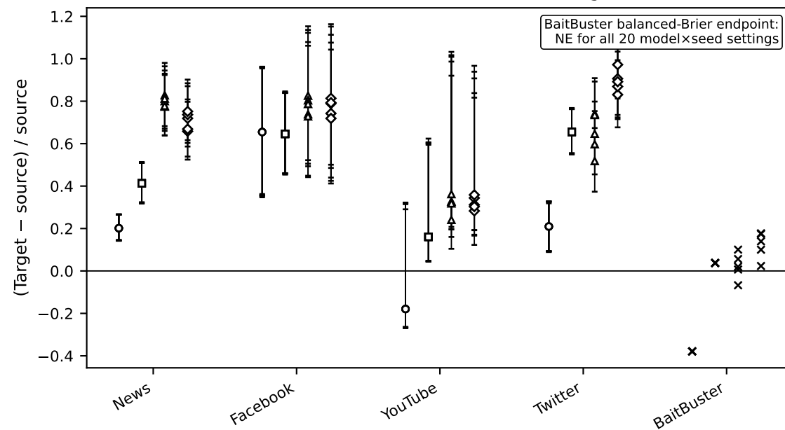
C. H1 relative balanced-Brier change
