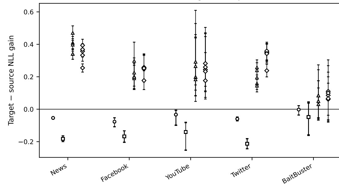
D. H2 calibration-gain transport
