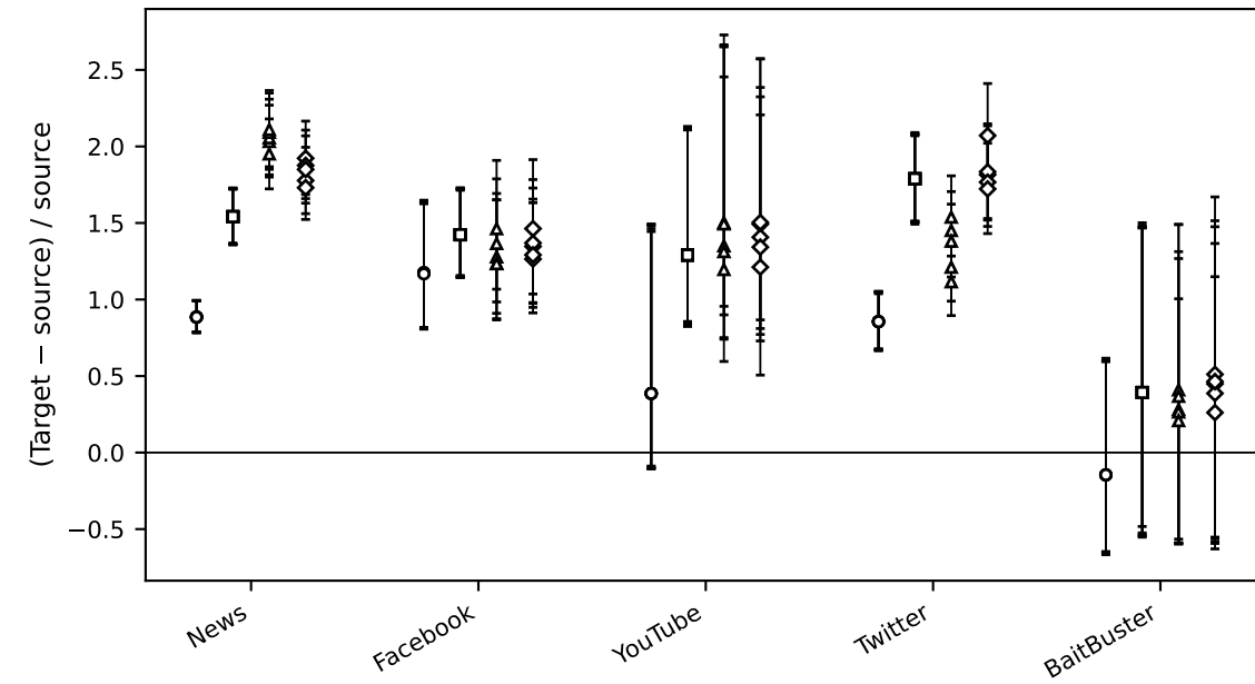
B. H1 relative NLL change
