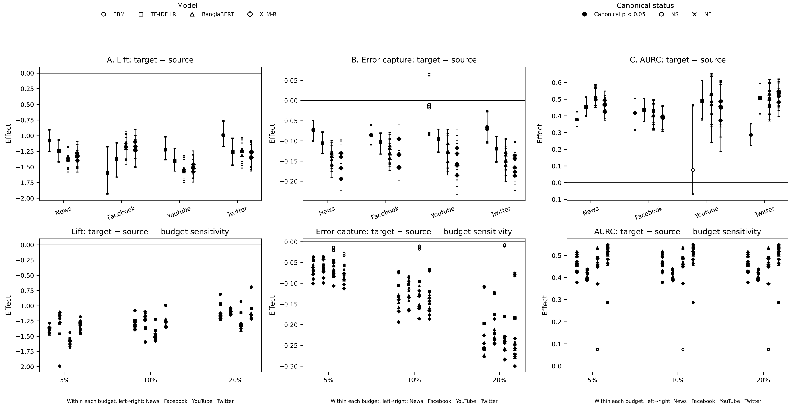
Figure 4. Fixed-budget operational degradation on BanglaClick 10% is primary; 5% and 20% are prespecified sensitivity budgets
