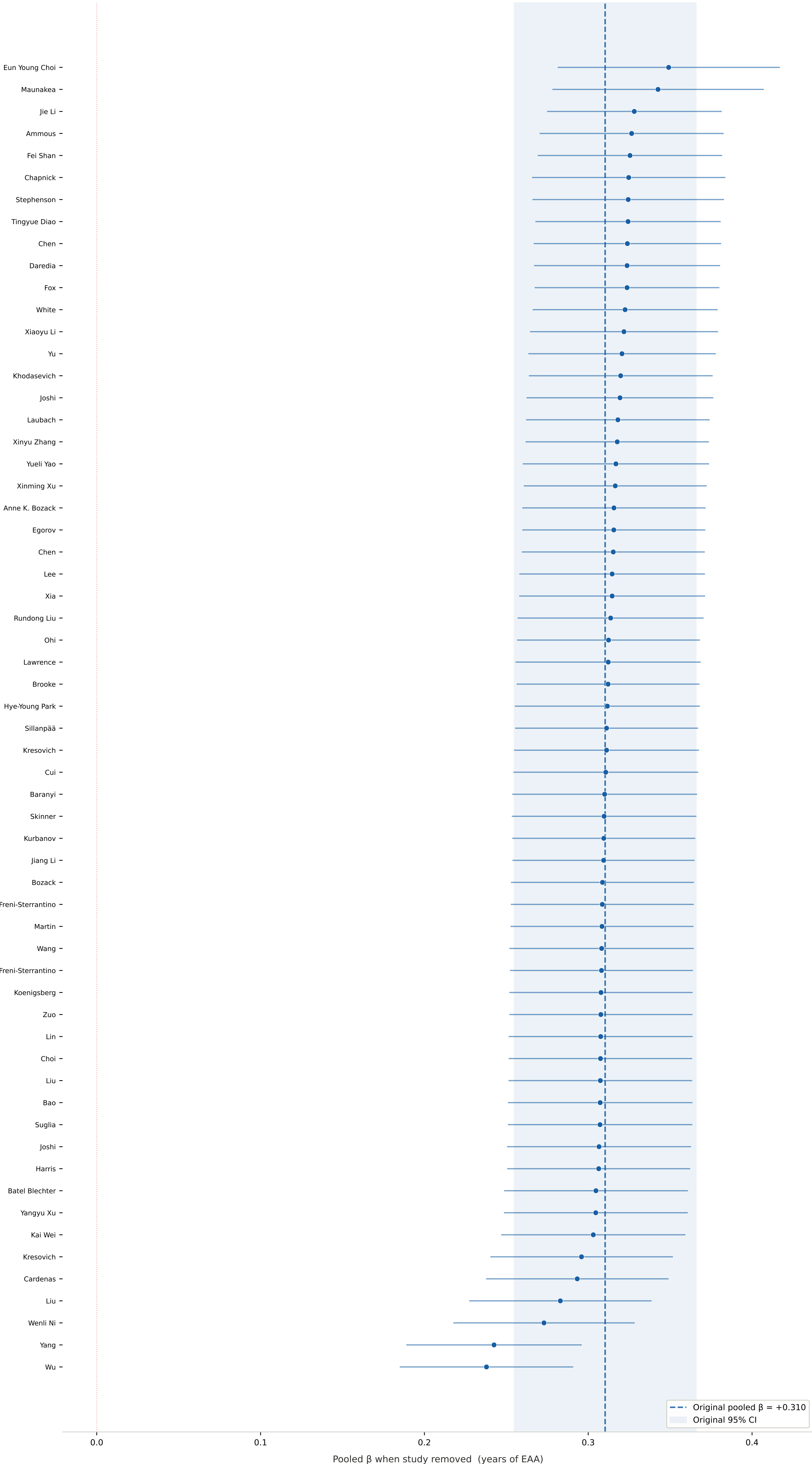
Leave-One-Out Sensitivity Analysis — Pool A (n = 60) Each point shows the pooled \beta when that study is excluded
