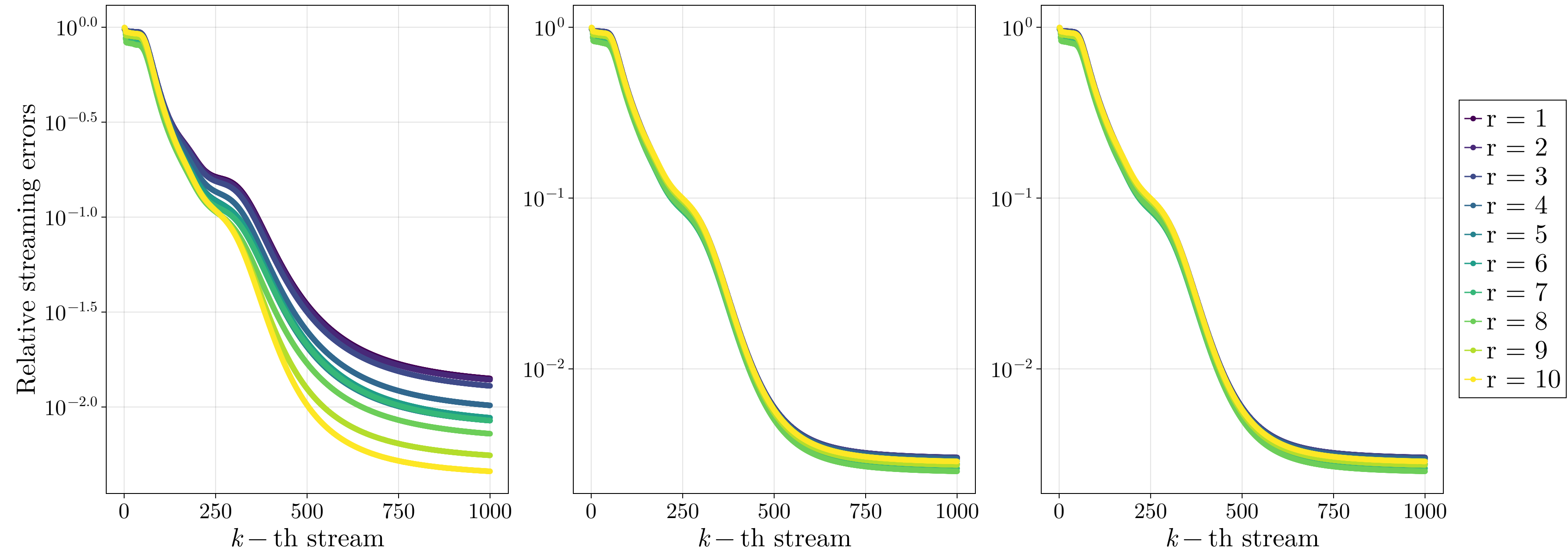
iQRRLS
