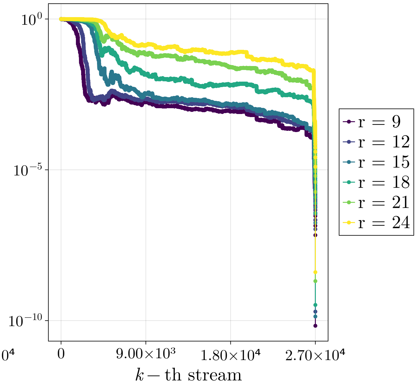
QRRLS
