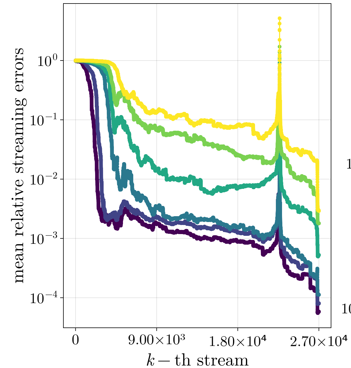
RLS
