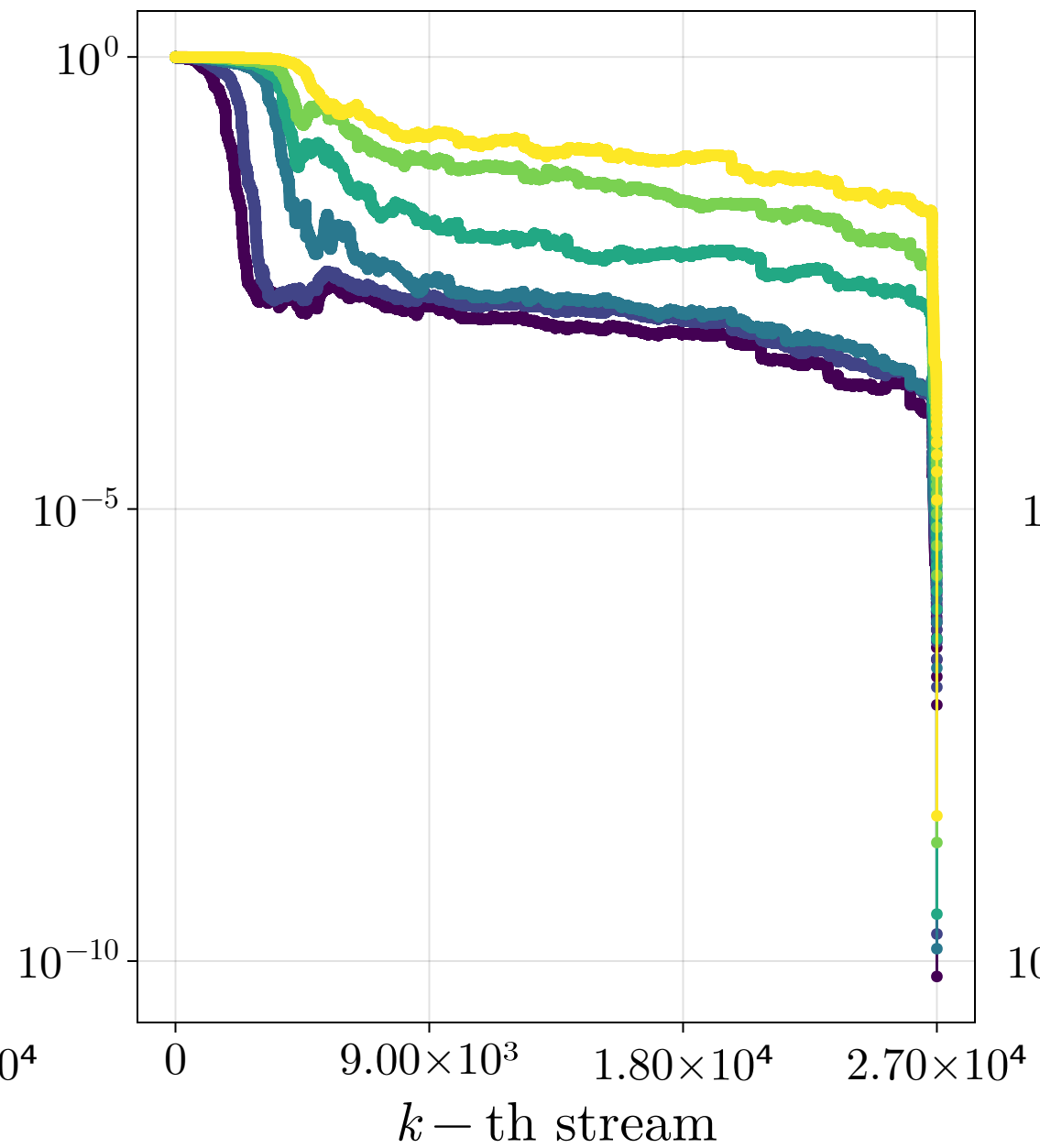
iQRRLS
