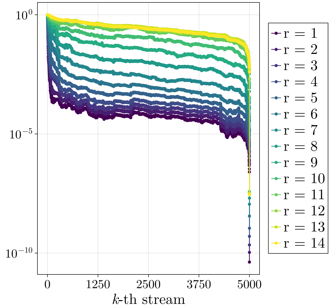
QRRLS
