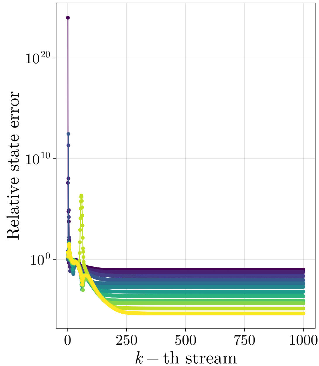
iQRRLS
