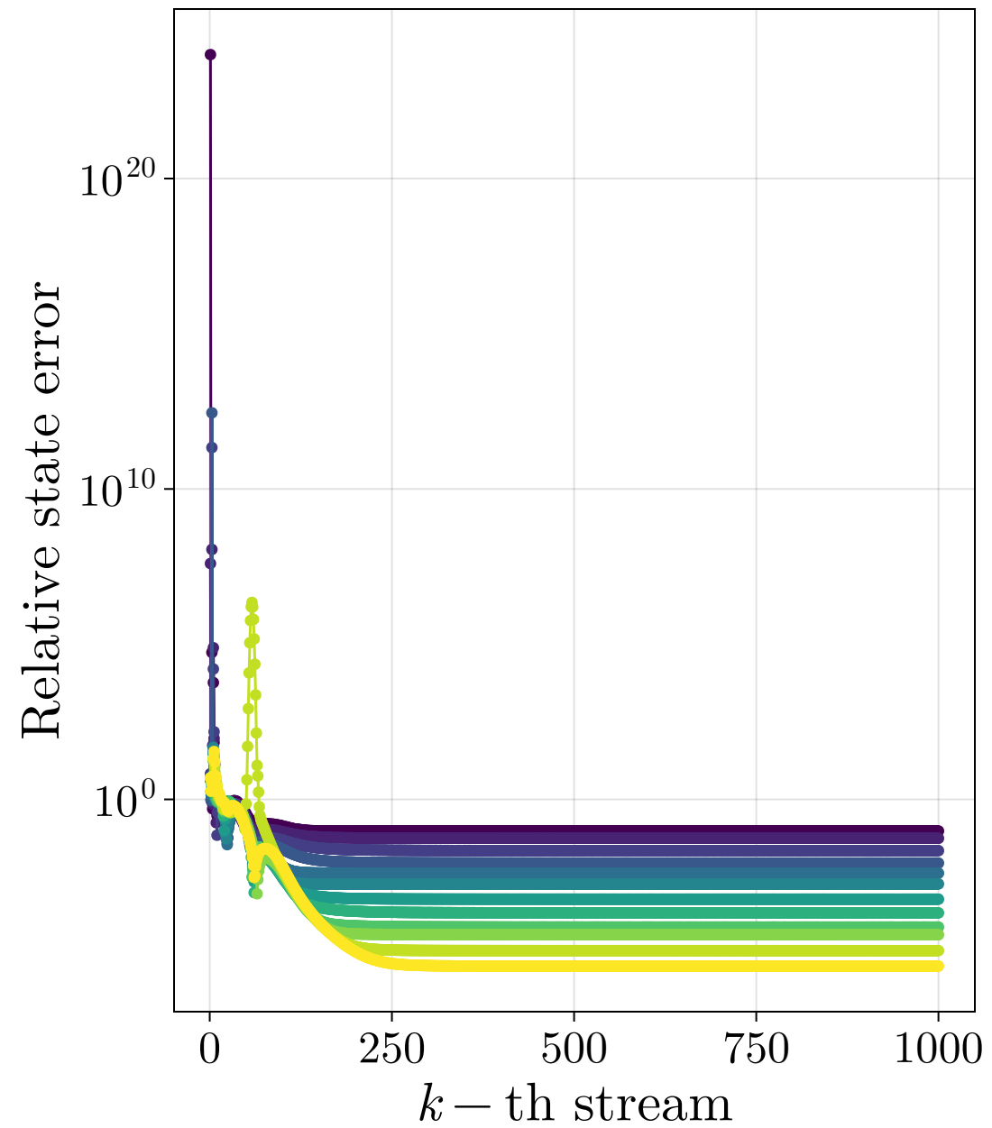
RLS
