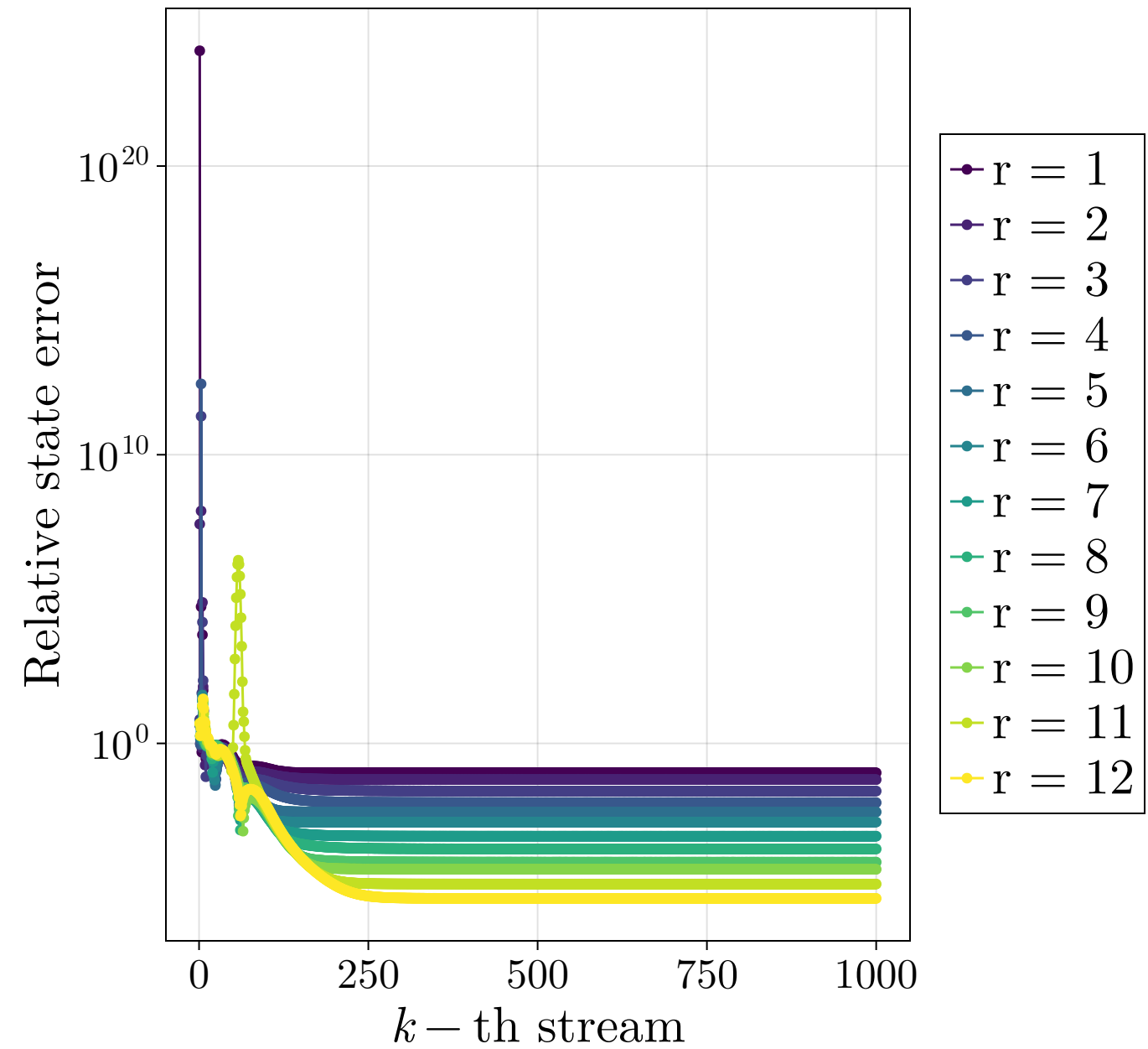
QRRLS
