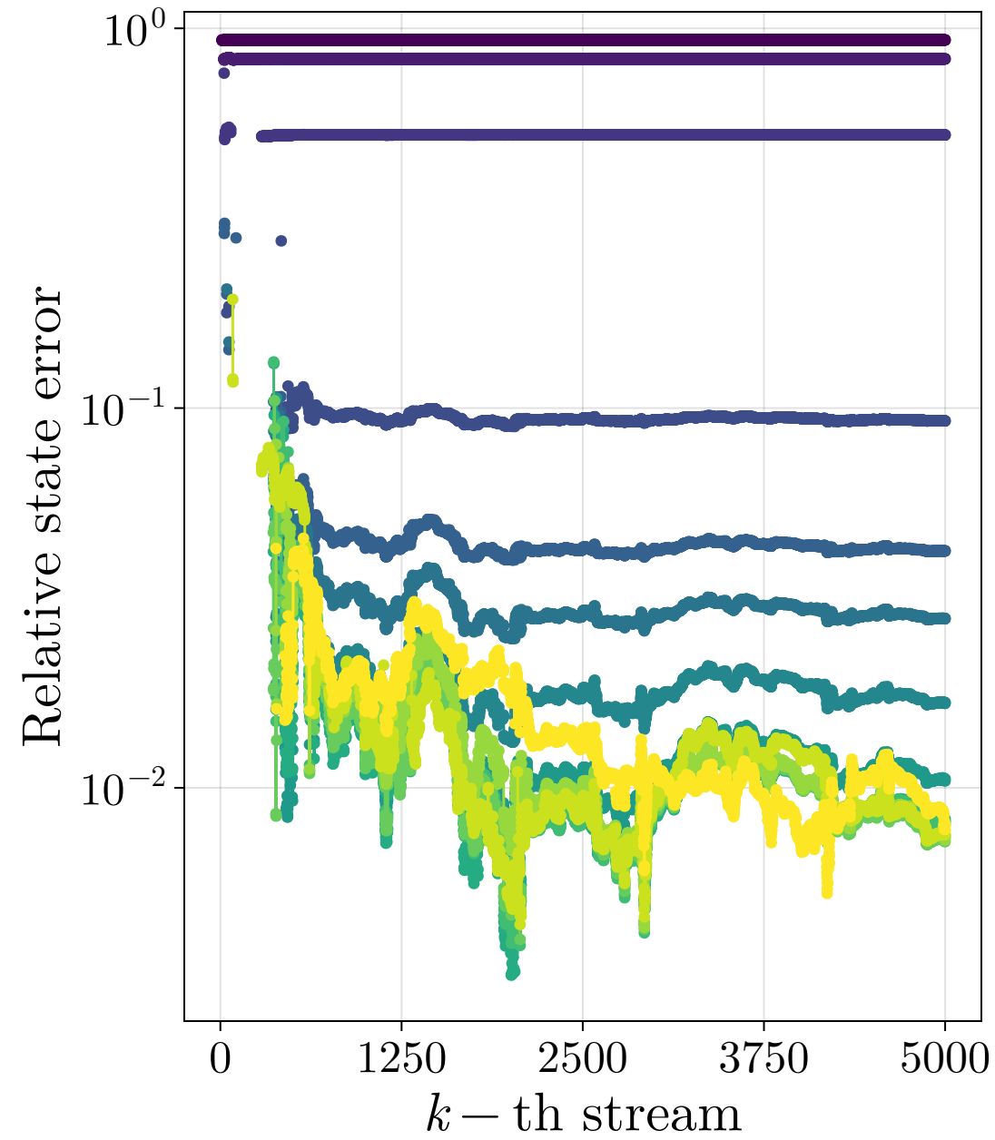
RLS
