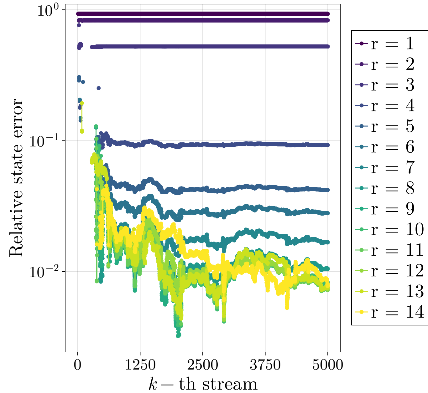
QRRLS
