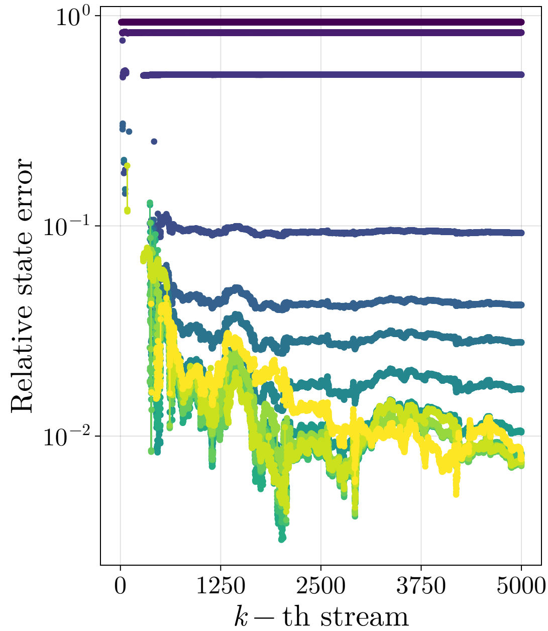
iQRRLS
