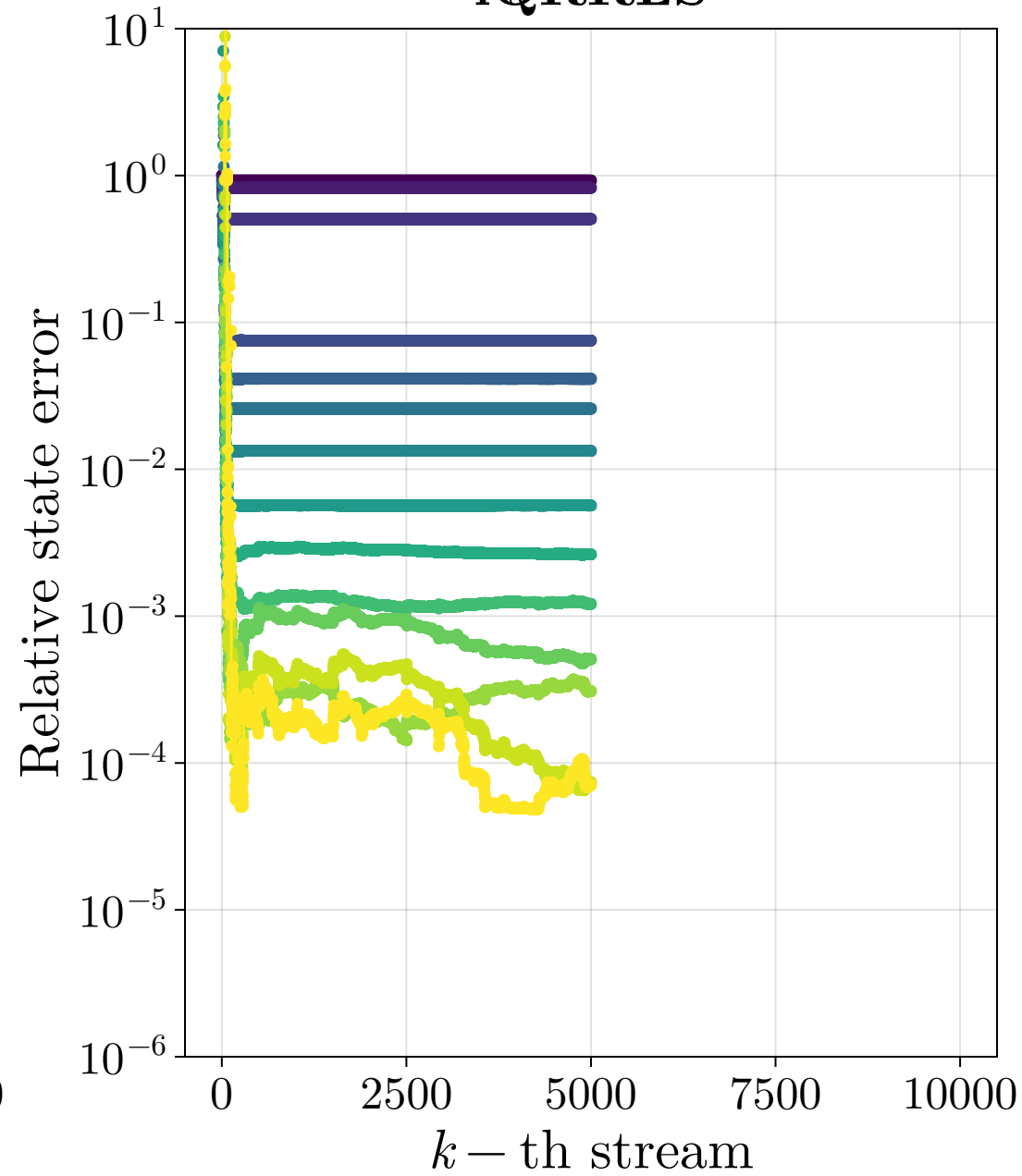
iQRRLS
