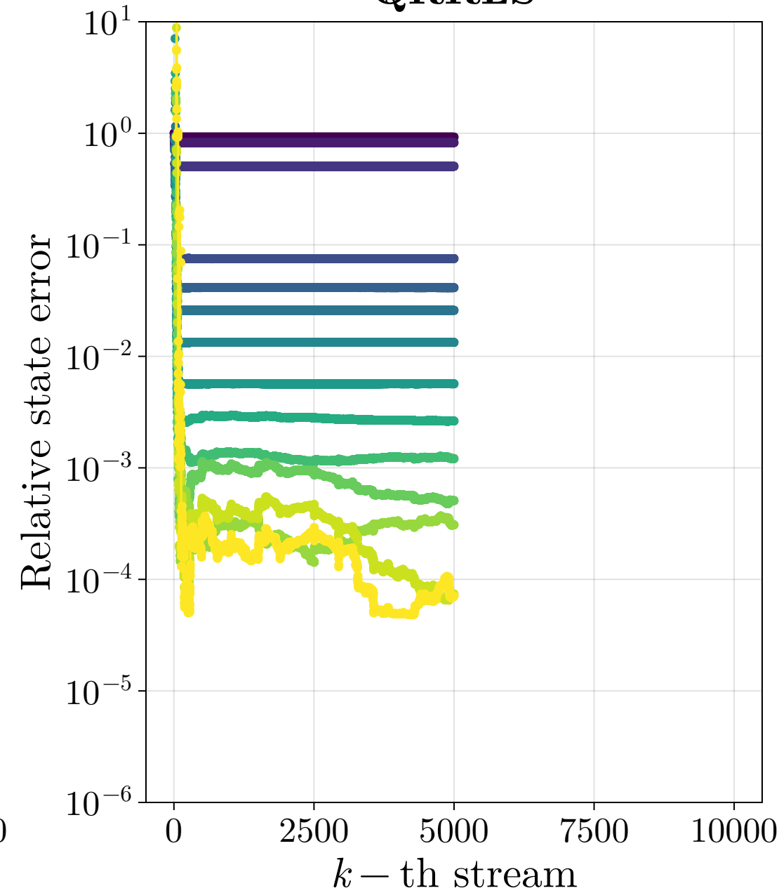
QRRLS
