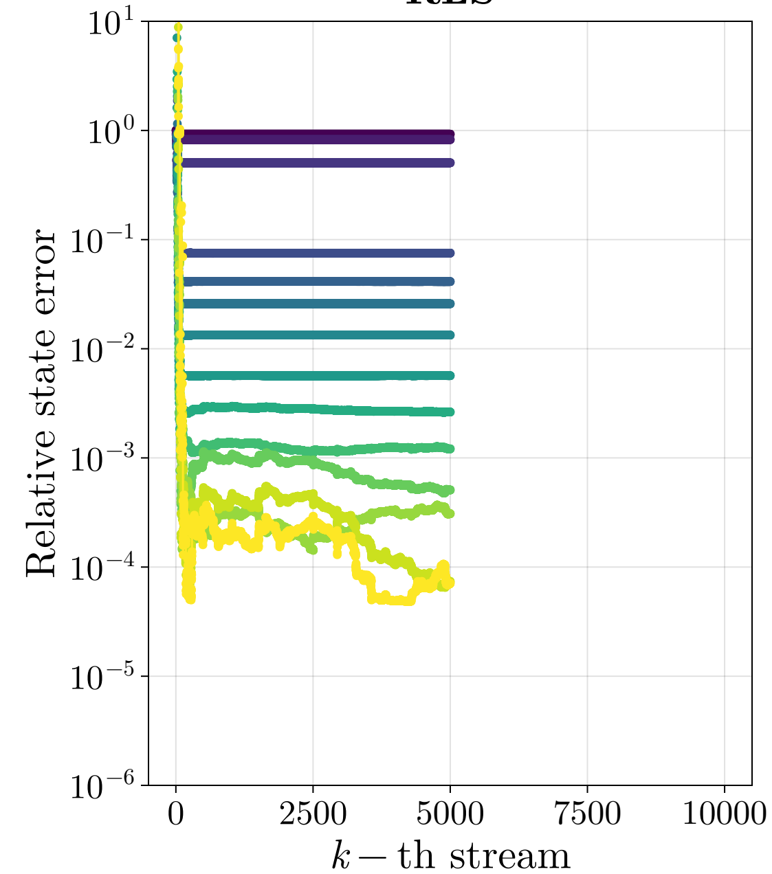
RLS
