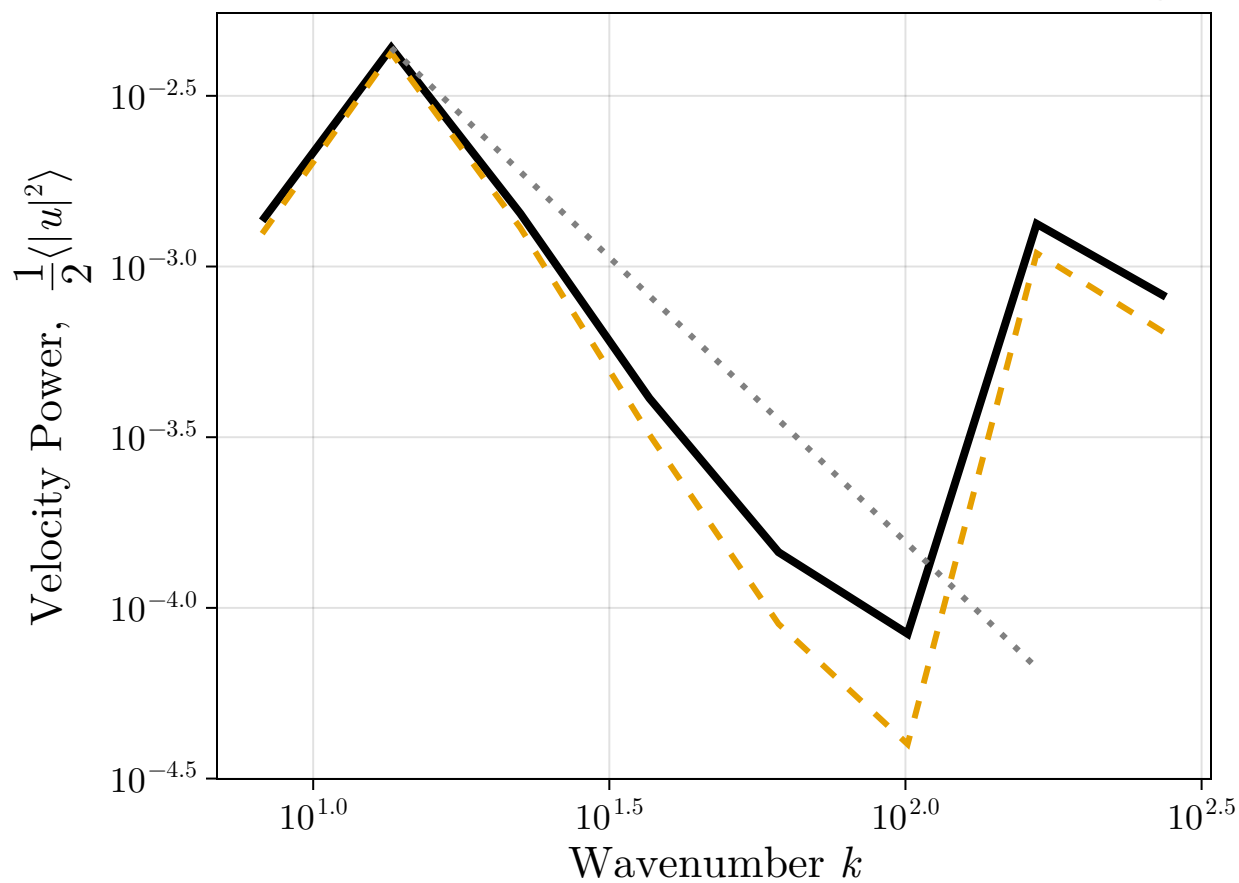
Velocity Power Spectrum - Training
