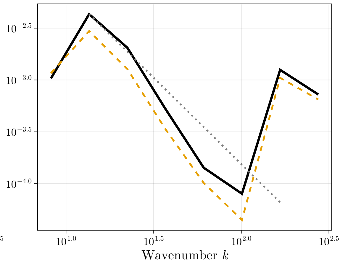
Velocity Power Spectrum - Testing
