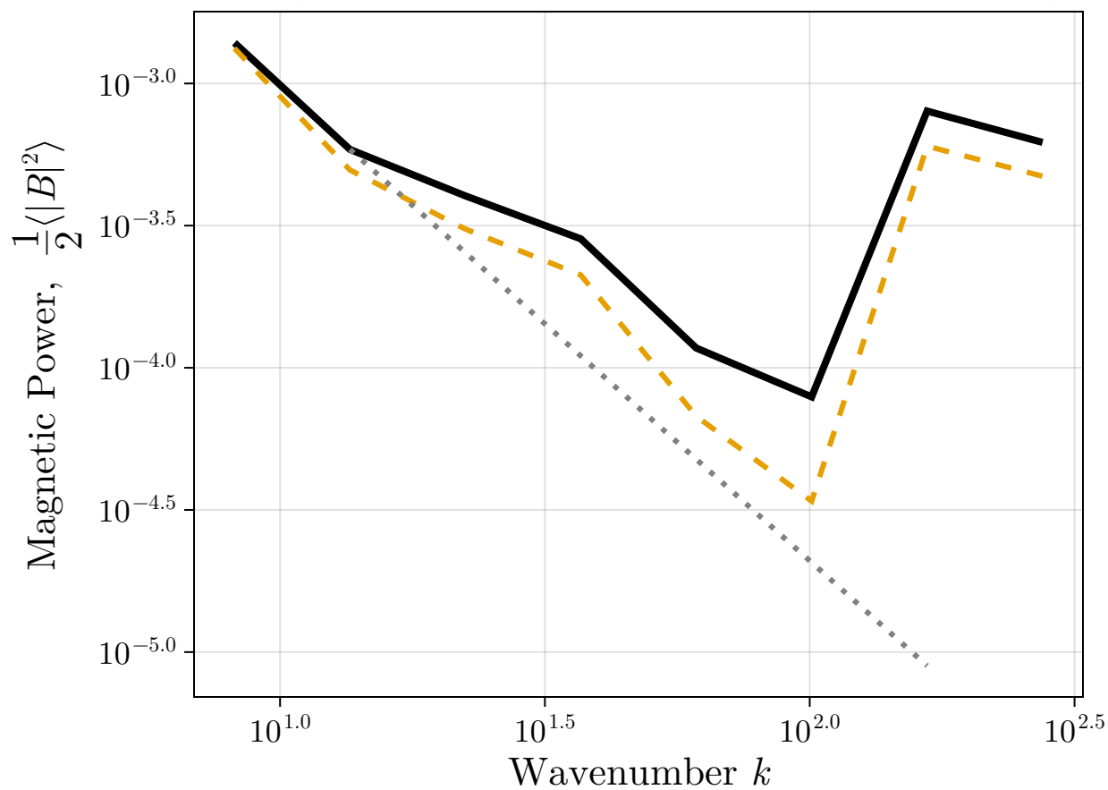
Magnetic Power Spectrum - Training
