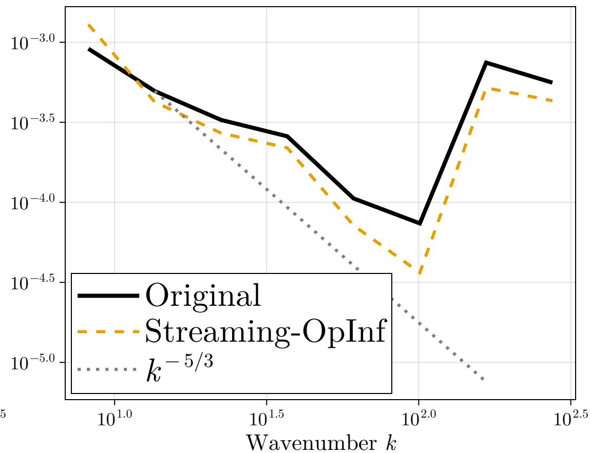
Magnetic Power Spectrum - Testing
