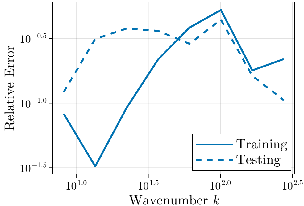
Velocity Power Spectrum Error
