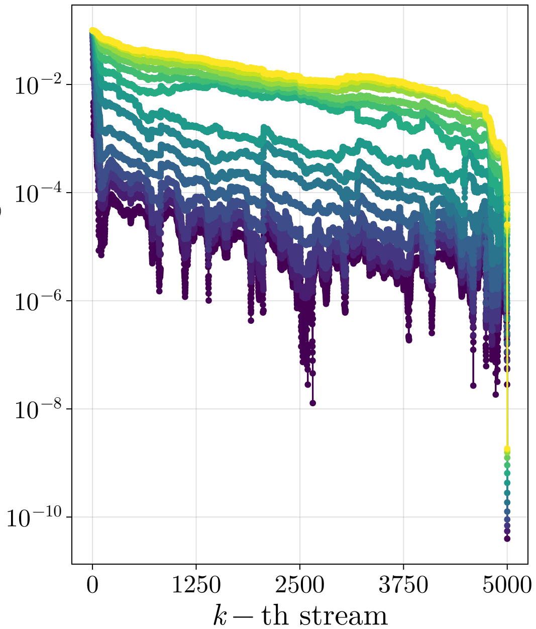
RLS
