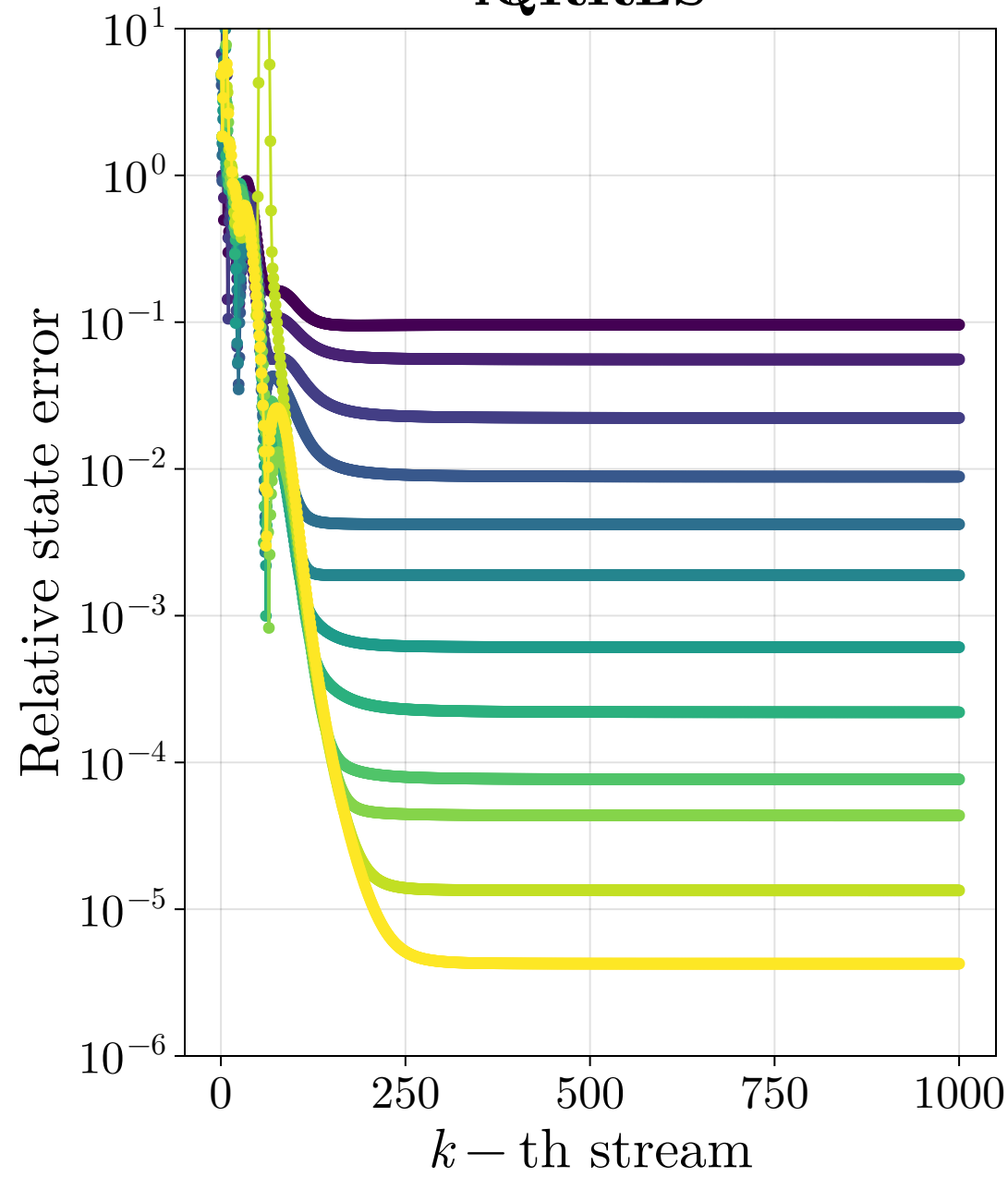
iQRRLS
