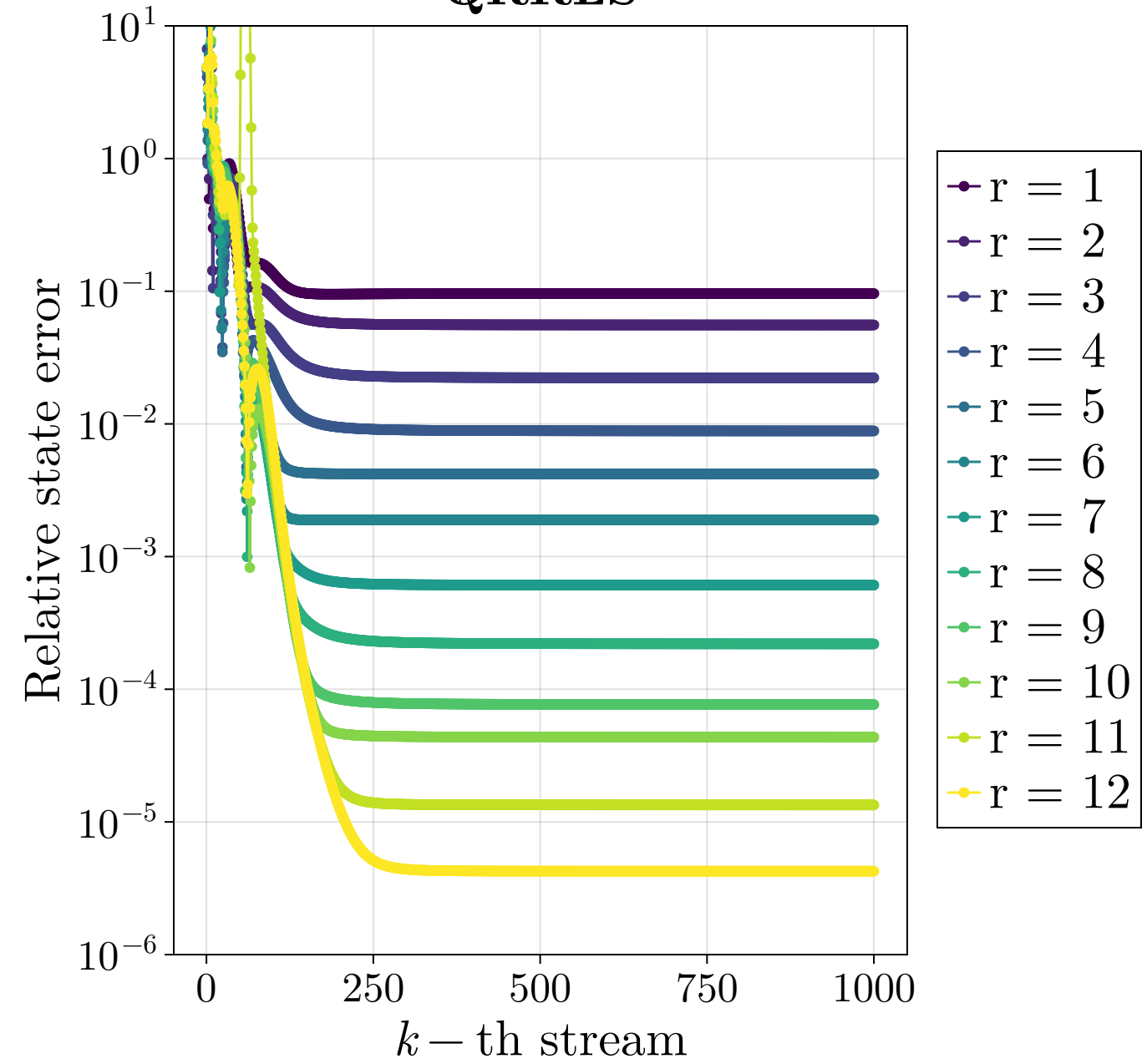
QRRLS
