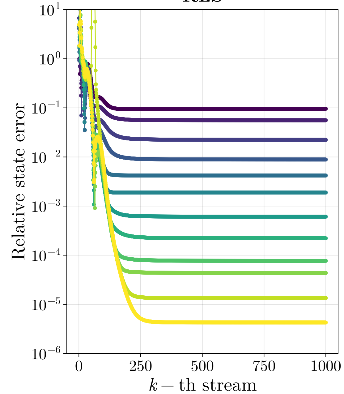
RLS
