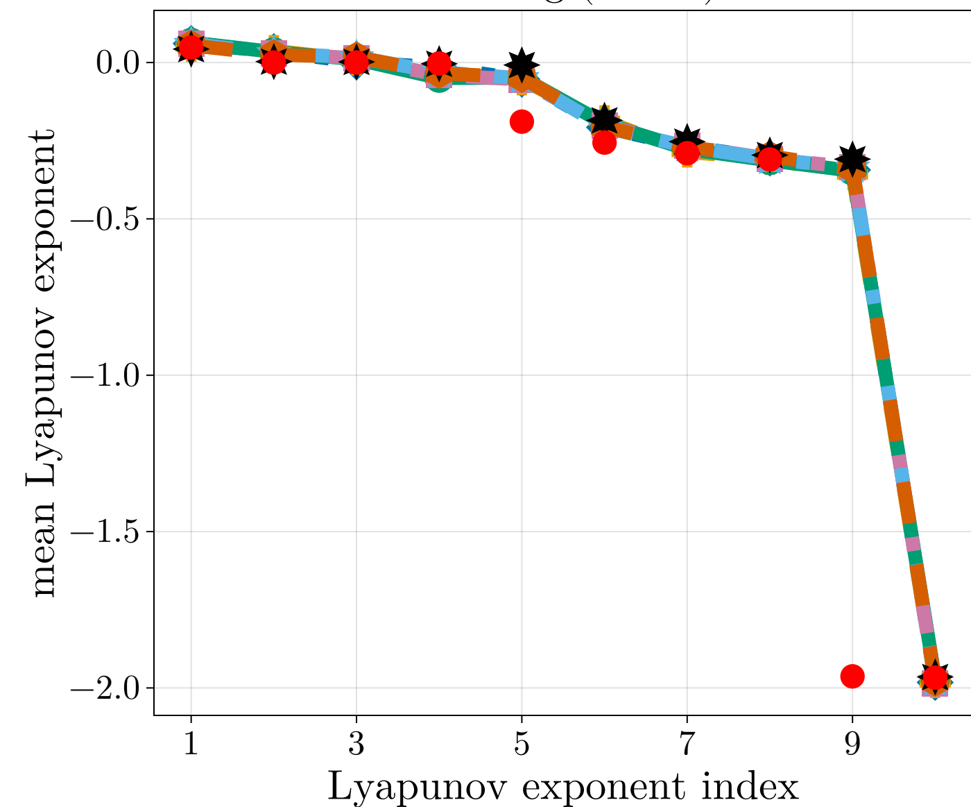
Training ( r=24 )
