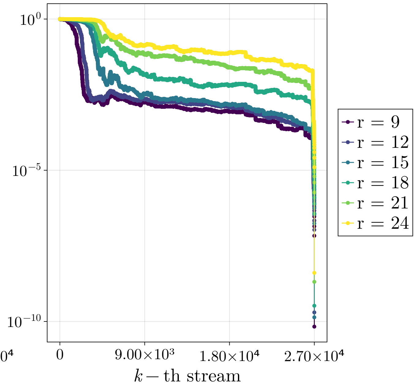
QRRLS
