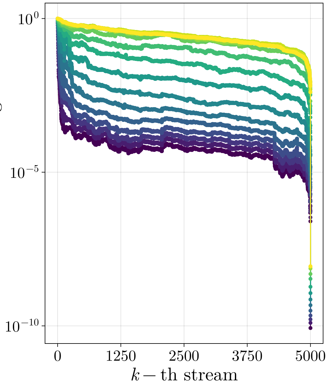
RLS
