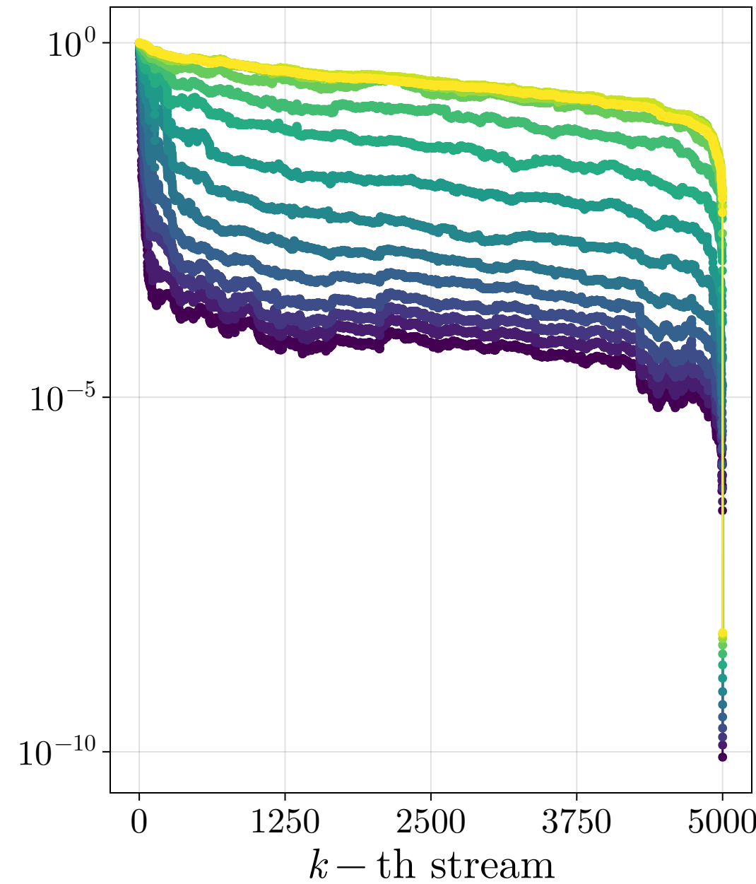
QRRLS
