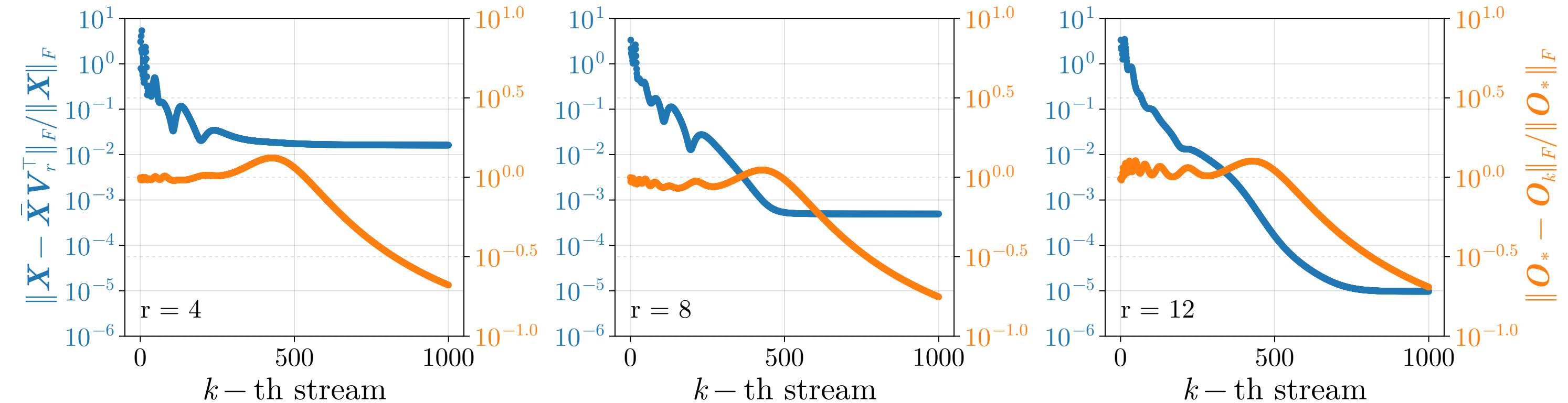
Relative State and Streaming Error per stream for different reduced dimensions
