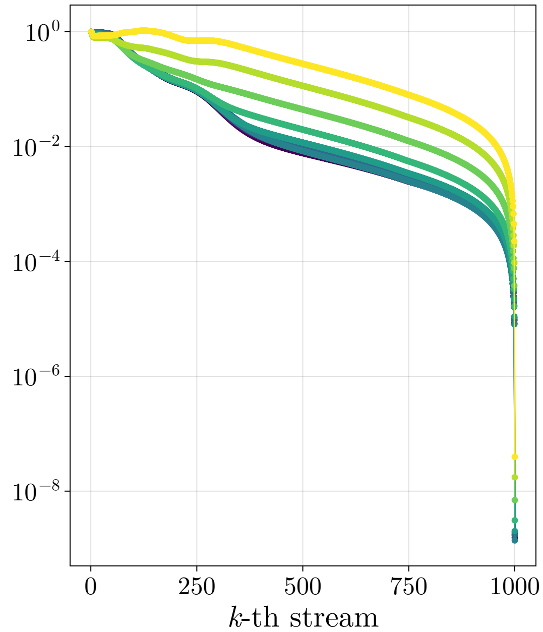
iQRRLS
