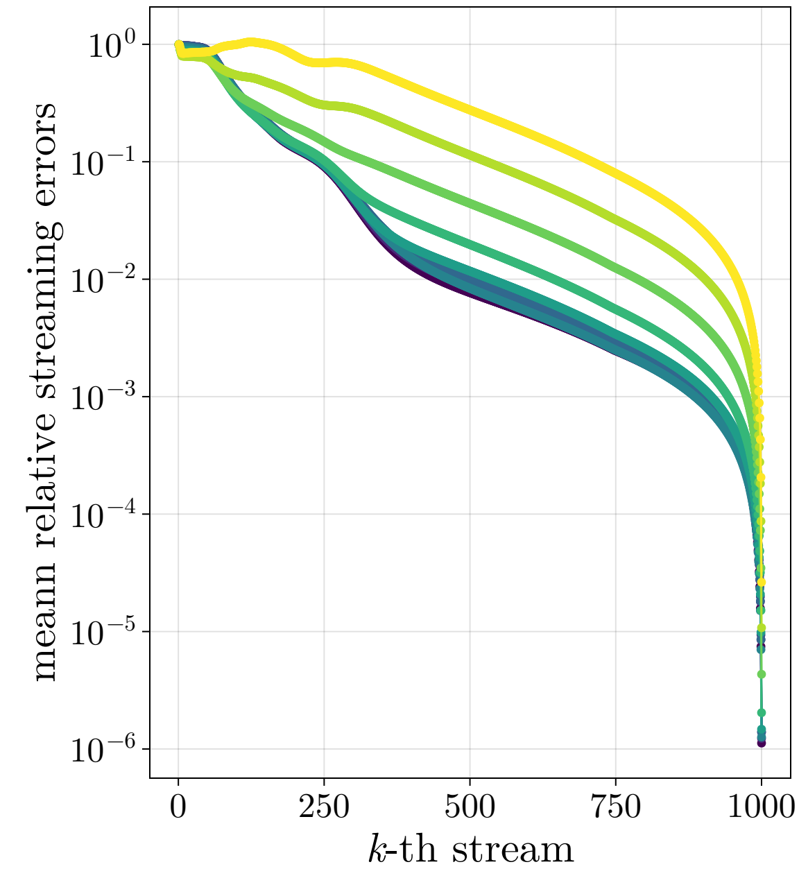
RLS
