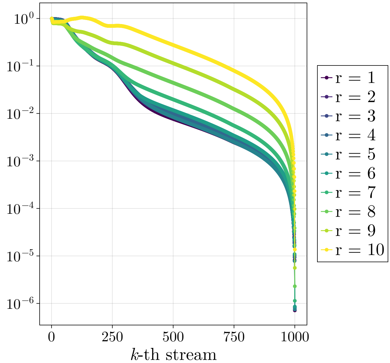
QRRLS
