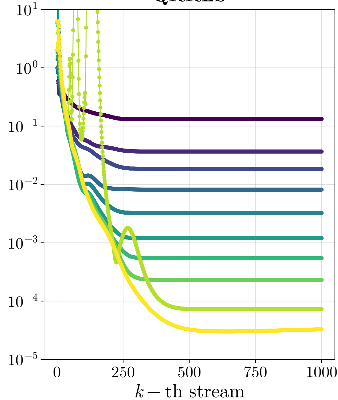
QRRLS
