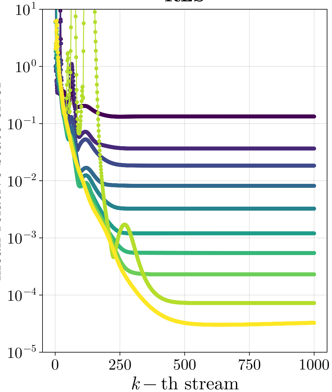
RLS
