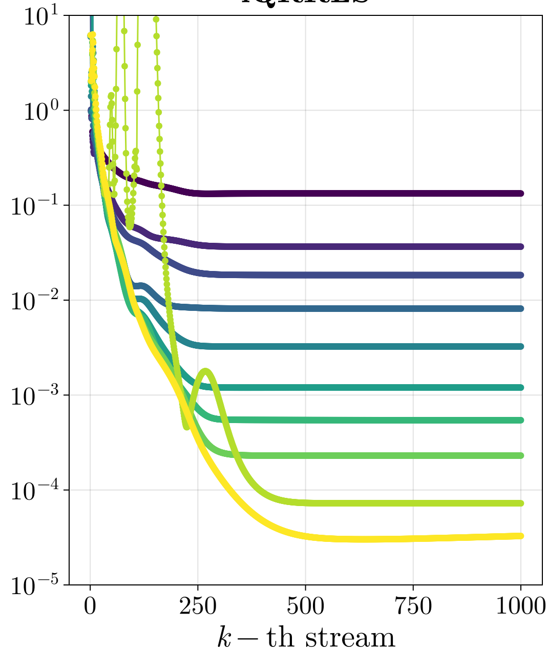
iQRRLS
