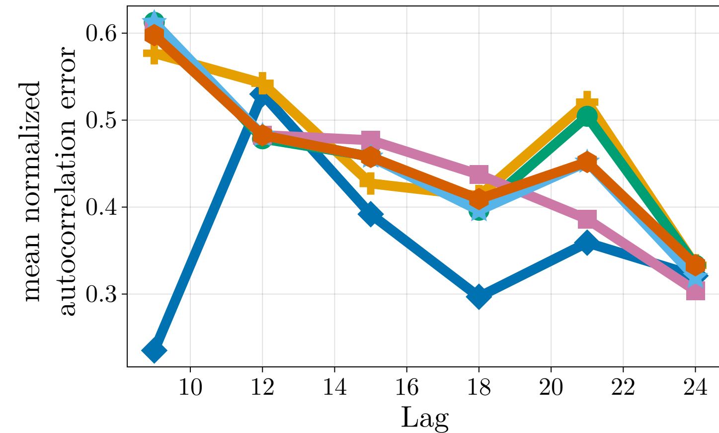
Training
