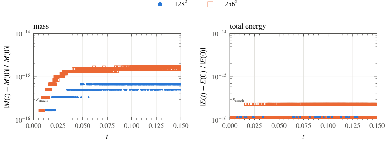
Figure 1: Relative change of the discrete mass and total energy at every time step, 128^2 (filled) and 256^2 (open) elements, N = 3 . Samples with no change at all (exact zeros) cannot be drawn on the logarithmic axis and are omitted; the totals move by single units in the last place, hence the discrete levels. Dotted: \varepsilon_{\text{mach}} .
